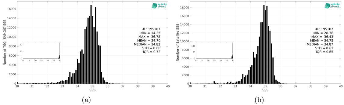
Figure 3: Histograms of SSS from TSG (SAMOS) (a) and CCI SSS L4 Merged-OI v4.41 - 30-day running (ESA) (b) considering all match-up pairs per bins of 0.1 over the Tropical Pacific Ocean Pi-MEP region and for the full satellite product period.
