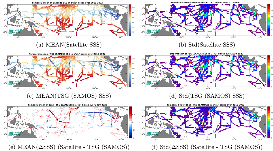
Figure 7: Temporal mean (left) and Std (right) of SSS from CCI SSS L4 Merged-OI v4.41 - 30-day running (ESA) (top), TSG (SAMOS) (middle), and of \Delta SSS (Satellite - TSG (SAMOS)). Only match-up pairs are used to generate these maps.
