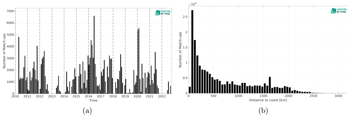
Figure 2: Number of match-ups between TSG (SAMOS) and CCI SSS L4 Merged-OI v4.41 - 30-day running (ESA) SSS as a function of time (a) and as function of the distance to coast (b) over the Tropical Pacific Ocean Pi-MEP region and for the full satellite product period.
