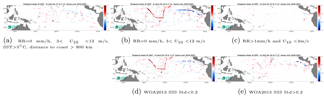
Figure 14: Temporal mean gridded over spatial boxes of size 1^\circ \times 1^\circ of \Delta SSS (CCI SSS L4 Merged-OI v4.41 - 30-day running (ESA) - TSG (SAMOS)) for 5 different subdatasets corresponding to:RR=0 mm/h, 3 < U_{10} < 12 m/s, SST > 5^\circ\text{C} , distance to coast > 800 km (a), RR=0 mm/h, 3 < U_{10} < 12 m/s (b), RR > 1 mm/h and U_{10} < 4 m/s (c), WOA2013 SSS Std < 0.2 (d), WOA2013 SSS Std > 0.2 (e).
