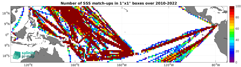
Figure 5: Number of SSS match-ups between TSG (LEGOS-DM) SSS and the CCI SSS L4 Merged-OI v4.41 - 30-day running (ESA) SSS product for the Tropical Pacific Ocean Pi-MEP region over 1^\circ \times 1^\circ boxes and for the full satellite product period.
