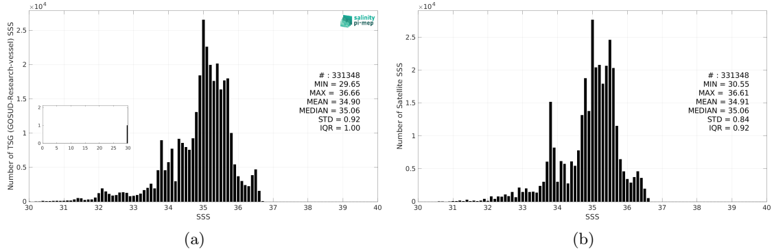
Figure 3: Histograms of SSS from TSG (GOSUD-Research-vessel) (a) and CCI SSS L4 Merged-OI v4.41 - 30-day running (ESA) (b) considering all match-up pairs per bins of 0.1 over the Tropical Pacific Ocean Pi-MEP region and for the full satellite product period.
