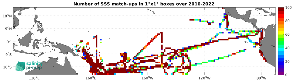
Figure 5: Number of SSS match-ups between TSG (GOSUD-Research-vessel) SSS and the CCI SSS L4 Merged-OI v4.41 - 30-day running (ESA) SSS product for the Tropical Pacific Ocean Pi-MEP region over 1^\circ \times 1^\circ boxes and for the full satellite product period.
