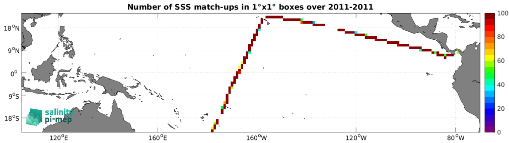
Figure 5: Number of SSS match-ups between TSG (CSIC-UTM) SSS and the CCI SSS L4 Merged-OI v4.41 - 30-day running (ESA) SSS product for the Tropical Pacific Ocean Pi-MEP region over 1^\circ \times 1^\circ boxes and for the full satellite product period.
