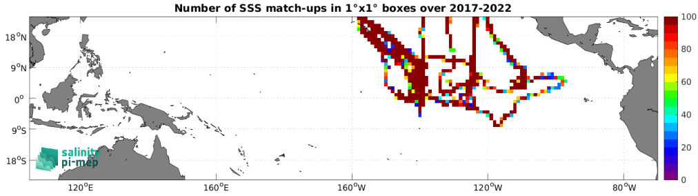
Figure 5: Number of SSS match-ups between Sailldrone SSS and the CCI SSS L4 Merged-OI v4.41 - 30-day running (ESA) SSS product for the Tropical Pacific Ocean Pi-MEP region over 1^\circ \times 1^\circ boxes and for the full satellite product period.
