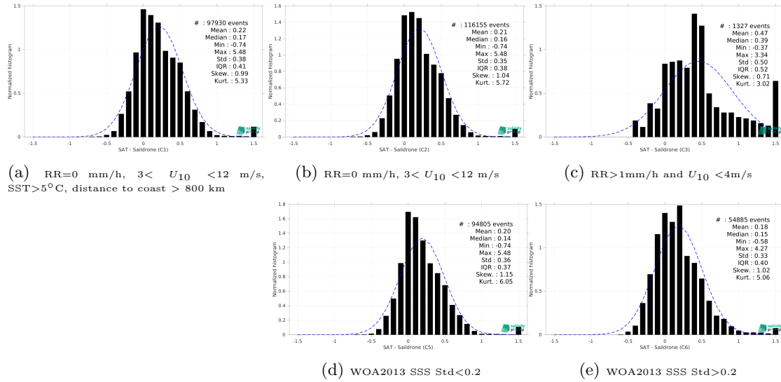
Figure 15: Normalized histogram of \Delta SSS (CCI SSS L4 Merged-OI v4.41 - 30-day running (ESA) - Saildrone) for 5 different subdatasets corresponding to: RR=0 mm/h, 3 < U_{10} < 12 m/s, SST>5°C, distance to coast > 800 km (a), RR=0 mm/h, 3 < U_{10} < 12 m/s (b), RR>1mm/h and U_{10} < 4 m/s (c), WOA2013 SSS Std<0.2 (d), WOA2013 SSS Std>0.2 (e).
