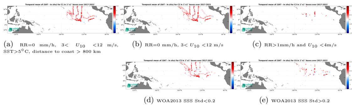
Figure 14: Temporal mean gridded over spatial boxes of size 1^\circ \times 1^\circ of \Delta SSS (CCI SSS L4 Merged-OI v4.41 - 30-day running (ESA) - Saildrone) for 5 different subdatasets corresponding to:RR=0 mm/h, 3 < U_{10} < 12 m/s, SST > 5^\circ\text{C} , distance to coast > 800 km (a), RR=0 mm/h, 3 < U_{10} < 12 m/s (b), RR > 1 mm/h and U_{10} < 4 m/s (c), WOA2013 SSS Std < 0.2 (d), WOA2013 SSS Std > 0.2 (e).
