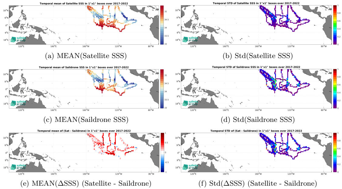
Figure 7: Temporal mean (left) and Std (right) of SSS from CCI SSS L4 Merged-OI v4.41 - 30-day running (ESA) (top), Saildrone (middle), and of \Delta SSS (Satellite - Saildrone). Only match-up pairs are used to generate these maps.
