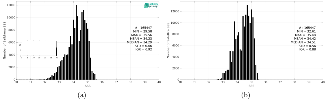
Figure 3: Histograms of SSS from Saildrone (a) and CCI SSS L4 Merged-OI v4.41 - 30-day running (ESA) (b) considering all match-up pairs per bins of 0.1 over the Tropical Pacific Ocean Pi-MEP region and for the full satellite product period.
