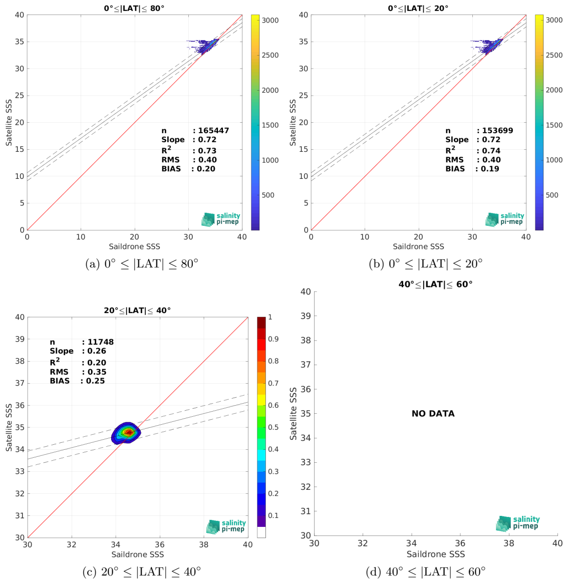
Figure 10: Contour maps of the concentration of CCI SSS L4 Merged-OI v4.41 - 30-day running (ESA) SSS (y-axis) versus Saildrone SSS (x-axis) at match-up pairs for different latitude bands. For each plot, the red line shows x=y . The black thin and dashed lines indicate a linear fit through the data cloud and the \pm 95\% confidence levels, respectively. The number match-up pairs n , the slope and R^2 coefficient of the linear fit, the root mean square (RMS) and the mean bias between satellite and in situ data are indicated for each latitude band in each plots.
