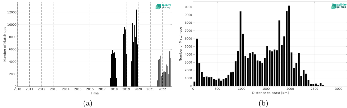
Figure 2: Number of match-ups between Saildrone and CCI SSS L4 Merged-OI v4.41 - 30-day running (ESA) SSS as a function of time (a) and as function of the distance to coast (b) over the Tropical Pacific Ocean Pi-MEP region and for the full satellite product period.
