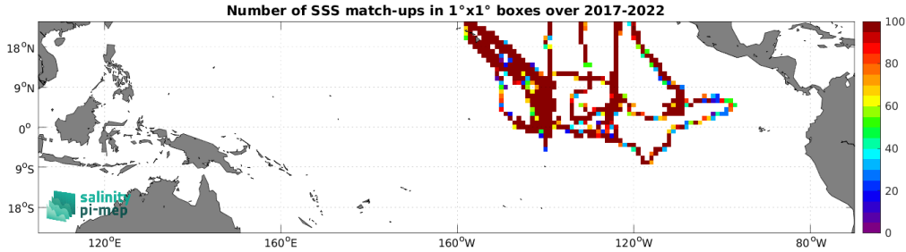
Figure 5: Number of SSS match-ups between Sailldrone SSS and the CCI SSS L4 Merged-OI v4.41 - 30-day running (ESA) SSS product for the Tropical Pacific Ocean Pi-MEP region over 1^\circ \times 1^\circ boxes and for the full satellite product period.
