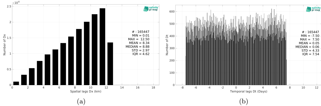
Figure 6: Histograms of the spatial (a) and temporal (b) lags between the location/time of the Sailldrone measurement and the date of the corresponding CCI SSS L4 Merged-OI v4.41 - 30-day running (ESA) SSS pixel.
