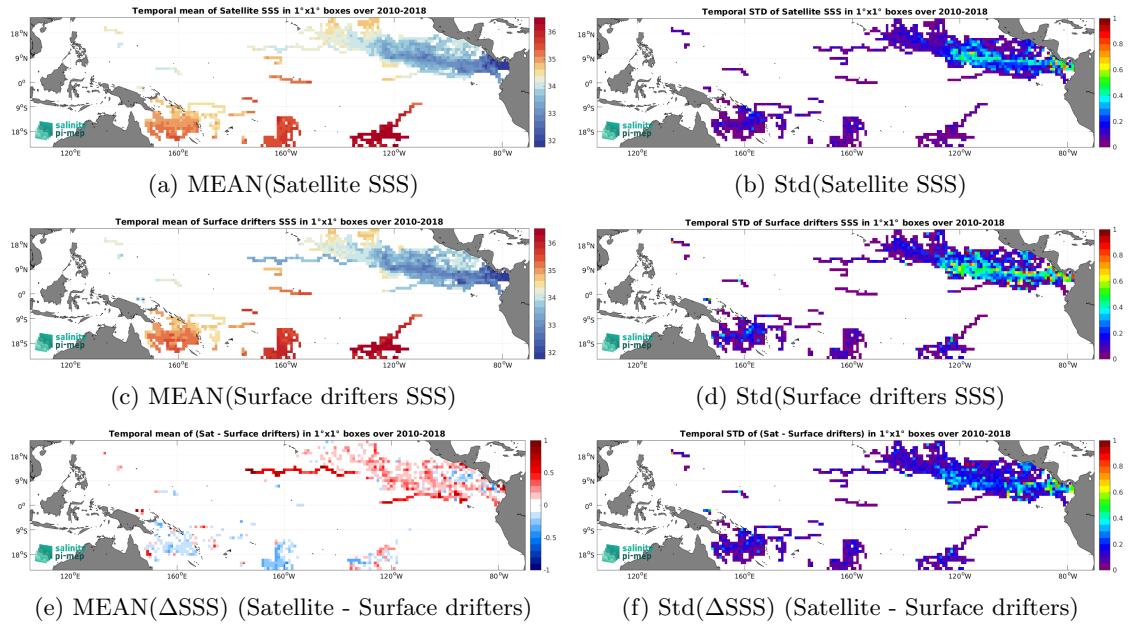
Figure 6: Temporal mean (left) and Std (right) of SSS from CCI SSS L4 Merged-OI v4.41 - 30-day running (ESA) (top), Surface drifters (middle), and of \Delta SSS (Satellite - Surface drifters). Only match-up pairs are used to generate these maps.
