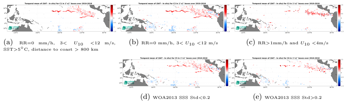
Figure 13: Temporal mean gridded over spatial boxes of size 1^\circ \times 1^\circ of \Delta SSS (CCI SSS L4 Merged-OI v4.41 - 30-day running (ESA) - Surface drifters) for 5 different subdatasets corresponding to:RR=0 mm/h, 3 < U_{10} < 12 m/s, SST > 5^\circ\text{C} , distance to coast > 800 km (a), RR=0 mm/h, 3 < U_{10} < 12 m/s (b), RR > 1 mm/h and U_{10} < 4 m/s (c), WOA2013 SSS Std < 0.2 (d), WOA2013 SSS Std > 0.2 (e).
