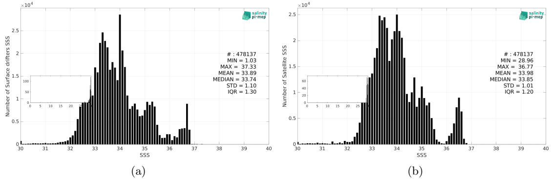
Figure 3: Histograms of SSS from Surface drifters (a) and CCI SSS L4 Merged-OI v4.41 - 30-day running (ESA) (b) considering all match-up pairs per bins of 0.1 over the Tropical Pacific Ocean Pi-MEP region and for the full satellite product period.
