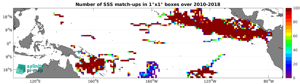
Figure 4: Number of SSS match-ups between Surface drifters SSS and the CCI SSS L4 Merged-OI v4.41 - 30-day running (ESA) SSS product for the Tropical Pacific Ocean Pi-MEP region over 1^\circ \times 1^\circ boxes and for the full satellite product period.
