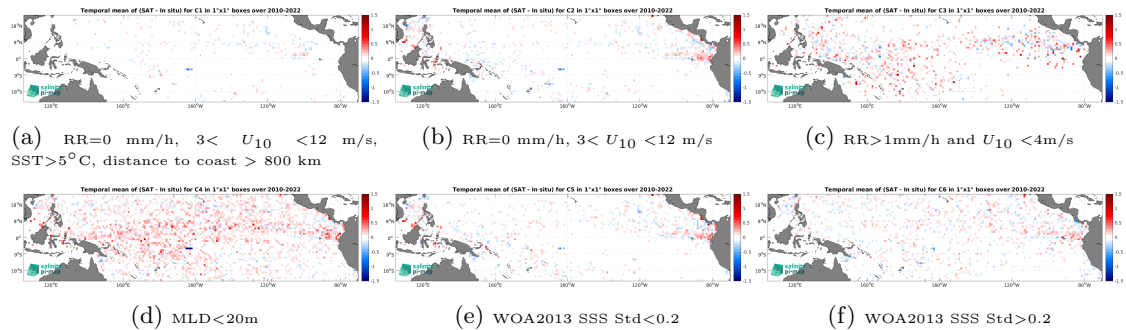
Figure 14: Temporal mean gridded over spatial boxes of size 1^\circ \times 1^\circ of \Delta SSS (CCI SSS L4 Merged-OI v4.41 - 30-day running (ESA) - Argo) for 6 different subdatasets corresponding to:RR=0 mm/h, 3 < U_{10} < 12 m/s, SST >5^\circ C, distance to coast > 800 km (a), RR=0 mm/h, 3 < U_{10} < 12 m/s (b), RR >1 mm/h and U_{10} < 4 m/s (c),MLD <20 m (d),WOA2013 SSS Std <0.2 (e),WOA2013 SSS Std >0.2 (f).
