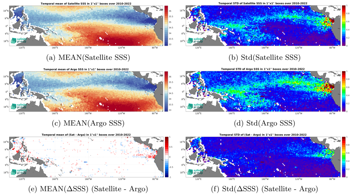
Figure 7: Temporal mean (left) and Std (right) of SSS from CCI SSS L4 Merged-OI v4.41 - 30-day running (ESA) (top), Argo (middle), and of \Delta SSS (Satellite - Argo). Only match-up pairs are used to generate these maps.
