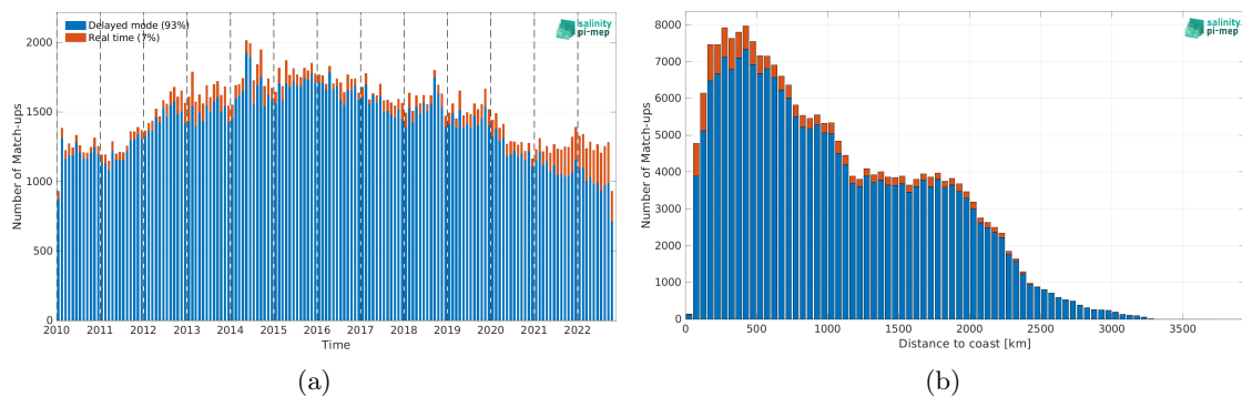
Figure 2: Number of match-ups between Argo and CCI SSS L4 Merged-OI v4.41 - 30-day running (ESA) SSS as a function of time (a) and as function of the distance to coast (b) over the Tropical Pacific Ocean Pi-MEP region and for the full satellite product period.
