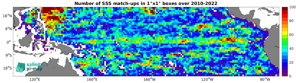
Figure 5: Number of SSS match-ups between Argo SSS and the CCI SSS L4 Merged-OI v4.41 - 30-day running (ESA) SSS product for the Tropical Pacific Ocean Pi-MEP region over 1^\circ \times 1^\circ boxes and for the full satellite product period.
