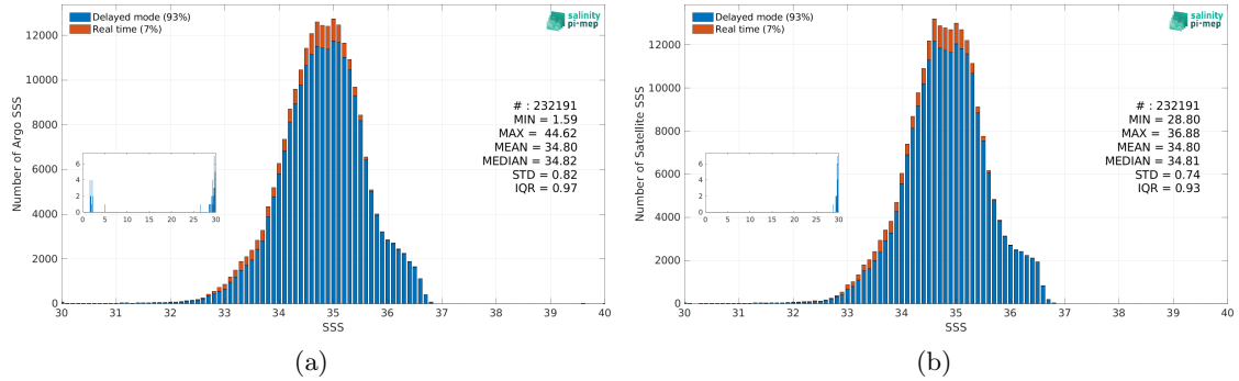
Figure 3: Histograms of SSS from Argo (a) and CCI SSS L4 Merged-OI v4.41 - 30-day running (ESA) (b) considering all match-up pairs per bins of 0.1 over the Tropical Pacific Ocean Pi-MEP region and for the full satellite product period.
