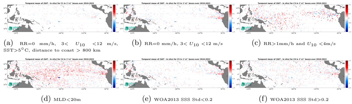
Figure 14: Temporal mean gridded over spatial boxes of size 1^\circ \times 1^\circ of \Delta SSS (CCI SSS L4 Merged-OI v4.41 - 30-day running (ESA) - Argo) for 6 different subdatasets corresponding to:RR=0 mm/h, 3 < U_{10} < 12 m/s, SST > 5^\circ\text{C} , distance to coast > 800 km (a), RR=0 mm/h, 3 < U_{10} < 12 m/s (b), RR > 1 mm/h and U_{10} < 4 m/s (c),MLD < 20 m (d),WOA2013 SSS Std < 0.2 (e),WOA2013 SSS Std > 0.2 (f).
