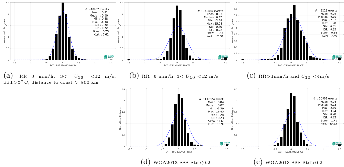
Figure 13: Normalized histogram of \Delta\text{SSS} (CCI SSS L4 Merged-OI v4.4 - 7-day running (ESA) - TSG (SAMOS)) for 5 different subdatasets corresponding to: RR=0 mm/h, 3 < U_{10} < 12 m/s, SST>5°C, distance to coast > 800 km (a), RR=0 mm/h, 3 < U_{10} < 12 m/s (b), RR>1mm/h and U_{10} < 4 m/s (c), WOA2013 SSS Std<0.2 (d), WOA2013 SSS Std>0.2 (e).
