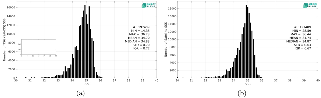
Figure 2: Histograms of SSS from TSG (SAMOS) (a) and CCI SSS L4 Merged-OI v4.4 - 7-day running (ESA) (b) considering all match-up pairs per bins of 0.1 over the Tropical Pacific Ocean Pi-MEP region and for the full satellite product period.
