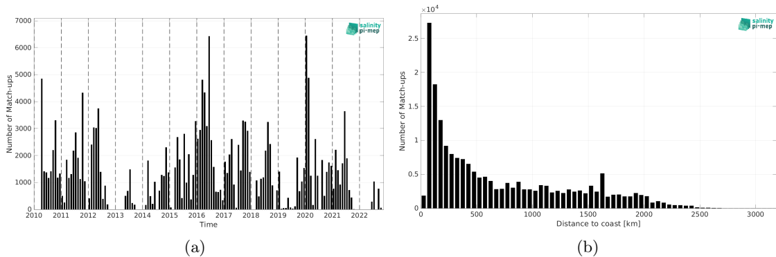
Figure 1: Number of match-ups between TSG (SAMOS) and CCI SSS L4 Merged-OI v4.4 - 7-day running (ESA) SSS as a function of time (a) and as function of the distance to coast (b) over the Tropical Pacific Ocean Pi-MEP region and for the full satellite product period.
