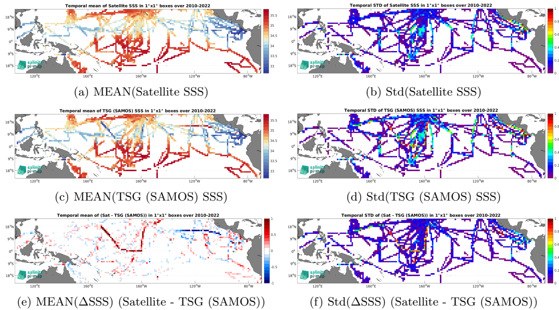
Figure 6: Temporal mean (left) and Std (right) of SSS from CCI SSS L4 Merged-OI v4.4 - 7-day running (ESA) (top), TSG (SAMOS) (middle), and of \Delta SSS (Satellite - TSG (SAMOS)). Only match-up pairs are used to generate these maps.
