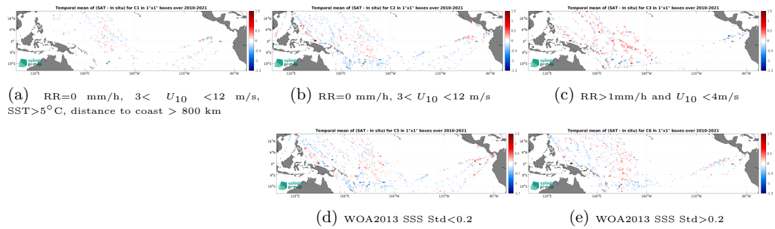
Figure 12: Temporal mean gridded over spatial boxes of size 1^\circ \times 1^\circ of \Delta SSS (CCI SSS L4 Merged-OI v4.4 - 7-day running (ESA) - TSG (LEGOS-DM)) for 5 different subdatasets corresponding to: RR=0 mm/h, 3 < U_{10} < 12 m/s, SST > 5^\circ\text{C} , distance to coast > 800 km (a), RR=0 mm/h, 3 < U_{10} < 12 m/s (b), RR > 1 mm/h and U_{10} < 4 m/s (c), WOA2013 SSS Std < 0.2 (d), WOA2013 SSS Std > 0.2 (e).
