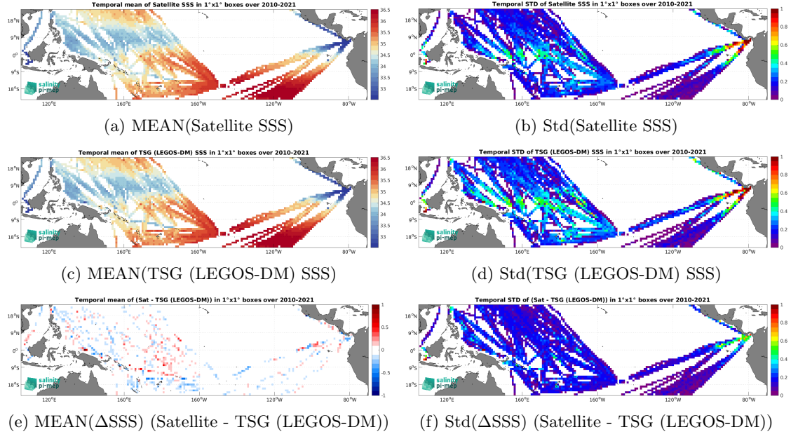
Figure 6: Temporal mean (left) and Std (right) of SSS from CCI SSS L4 Merged-OI v4.4 - 7-day running (ESA) (top), TSG (LEGOS-DM) (middle), and of \Delta SSS (Satellite - TSG (LEGOS-DM)). Only match-up pairs are used to generate these maps.
