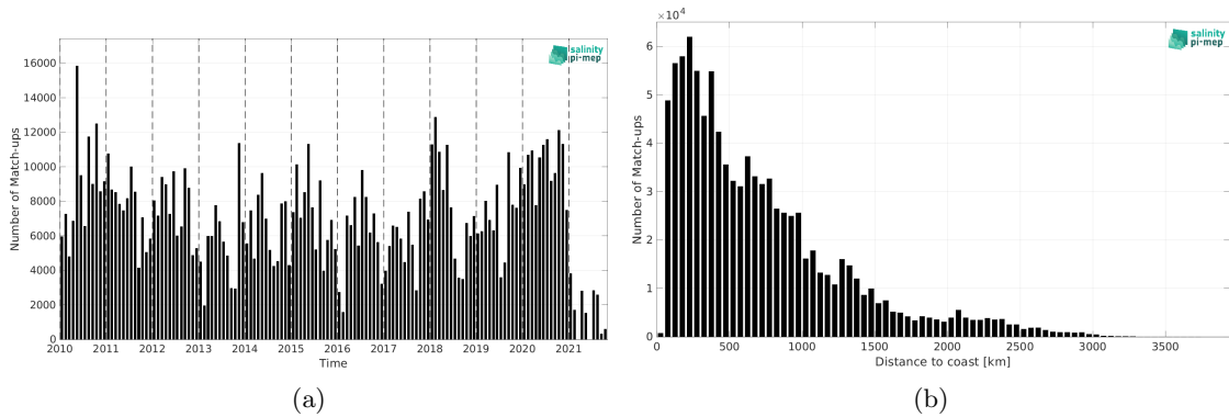
Figure 1: Number of match-ups between TSG (LEGOS-DM) and CCI SSS L4 Merged-OI v4.4 - 7-day running (ESA) SSS as a function of time (a) and as function of the distance to coast (b) over the Tropical Pacific Ocean Pi-MEP region and for the full satellite product period.
