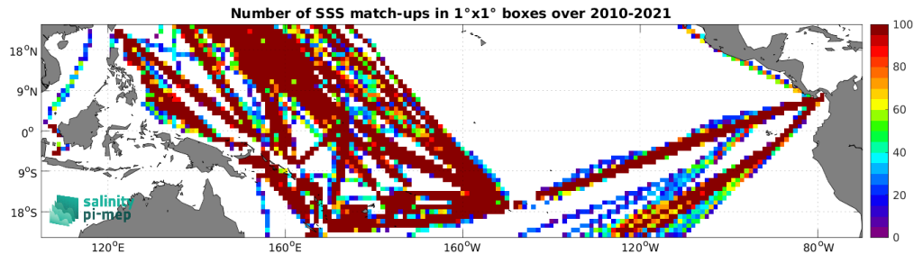
Figure 4: Number of SSS match-ups between TSG (LEGOS-DM) SSS and the CCI SSS L4 Merged-OI v4.4 - 7-day running (ESA) SSS product for the Tropical Pacific Ocean Pi-MEP region over 1^\circ \times 1^\circ boxes and for the full satellite product period.
