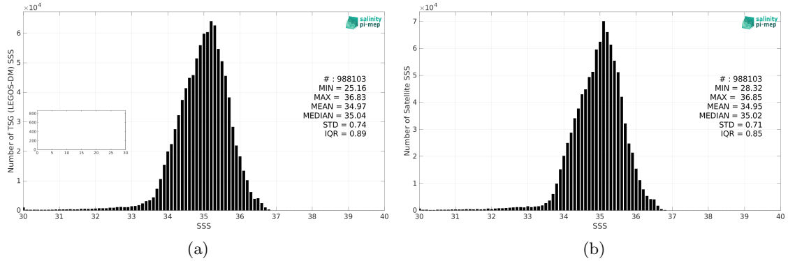
Figure 2: Histograms of SSS from TSG (LEGOS-DM) (a) and CCI SSS L4 Merged-OI v4.4 - 7-day running (ESA) (b) considering all match-up pairs per bins of 0.1 over the Tropical Pacific Ocean Pi-MEP region and for the full satellite product period.
