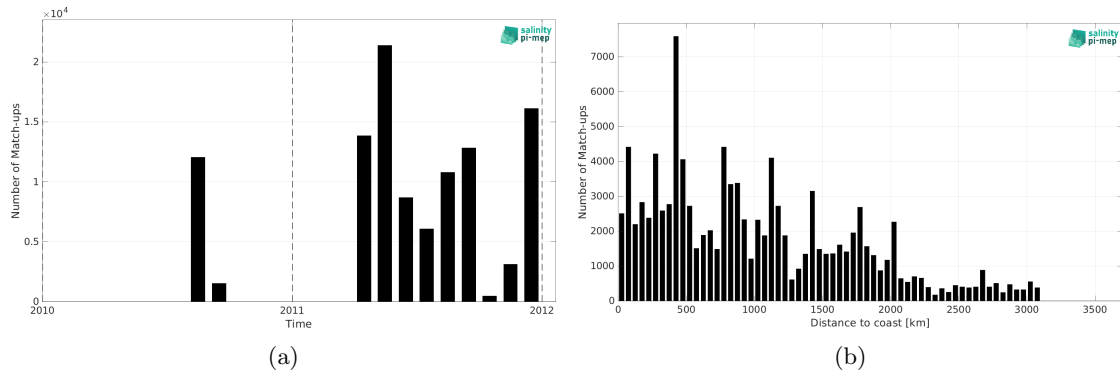
Figure 1: Number of match-ups between TSG (GOSUD-Sailing-ship) and CCI SSS L4 Merged-OI v4.4 - 7-day running (ESA) SSS as a function of time (a) and as function of the distance to coast (b) over the Tropical Pacific Ocean Pi-MEP region and for the full satellite product period.
