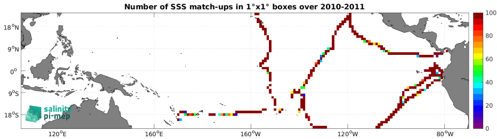
Figure 4: Number of SSS match-ups between TSG (GOSUD-Sailing-ship) SSS and the CCI SSS L4 Merged-OI v4.4 - 7-day running (ESA) SSS product for the Tropical Pacific Ocean Pi-MEP region over 1^\circ \times 1^\circ boxes and for the full satellite product period.
