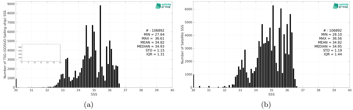
Figure 2: Histograms of SSS from TSG (GOSUD-Sailing-ship) (a) and CCI SSS L4 Merged-OI v4.4 - 7-day running (ESA) (b) considering all match-up pairs per bins of 0.1 over the Tropical Pacific Ocean Pi-MEP region and for the full satellite product period.
