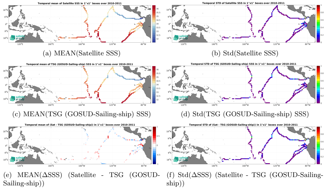
Figure 6: Temporal mean (left) and Std (right) of SSS from CCI SSS L4 Merged-OI v4.4 - 7-day running (ESA) (top), TSG (GOSUD-Sailing-ship) (middle), and of \Delta SSS (Satellite - TSG (GOSUD-Sailing-ship)). Only match-up pairs are used to generate these maps.
