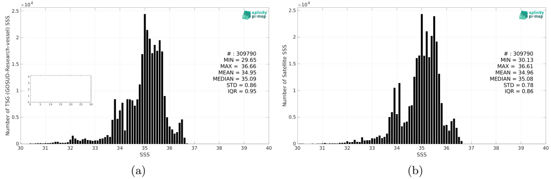
Figure 2: Histograms of SSS from TSG (GOSUD-Research-vessel) (a) and CCI SSS L4 Merged-OI v4.4 - 7-day running (ESA) (b) considering all match-up pairs per bins of 0.1 over the Tropical Pacific Ocean Pi-MEP region and for the full satellite product period.
