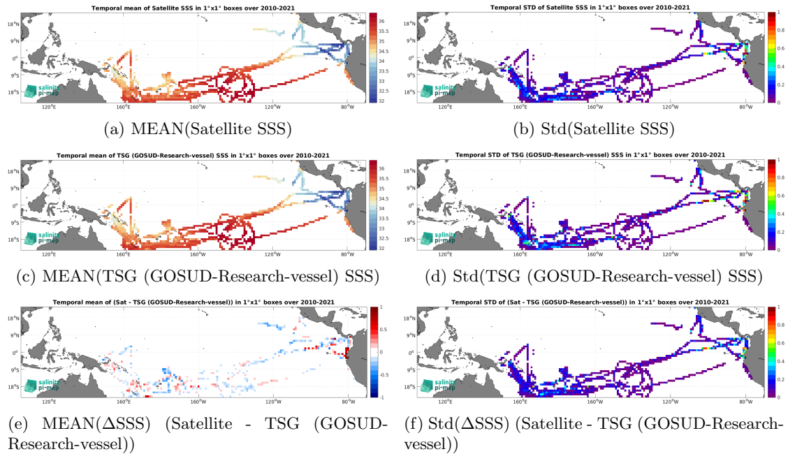
Figure 6: Temporal mean (left) and Std (right) of SSS from CCI SSS L4 Merged-OI v4.4 - 7-day running (ESA) (top), TSG (GOSUD-Research-vessel) (middle), and of \Delta SSS (Satellite - TSG (GOSUD-Research-vessel)). Only match-up pairs are used to generate these maps.
