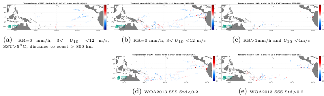
Figure 12: Temporal mean gridded over spatial boxes of size 1^{\circ}\times 1^{\circ} of \Delta SSS (CCI SSS L4 Merged-OI v4.4 - 7-day running (ESA) - TSG (GOSUD-Research-vessel)) for 5 different subdatasets corresponding to:RR=0 mm/h, 3 < U_{10} < 12 m/s, SST >5^{\circ}\text{C} , distance to coast > 800 km (a), RR=0 mm/h, 3 < U_{10} < 12 m/s (b), RR >1 mm/h and U_{10} < 4 m/s (c), WOA2013 SSS Std <0.2 (d), WOA2013 SSS Std >0.2 (e).
