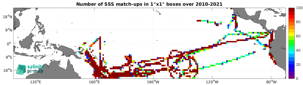
Figure 4: Number of SSS match-ups between TSG (GOSUD-Research-vessel) SSS and the CCI SSS L4 Merged-OI v4.4 - 7-day running (ESA) SSS product for the Tropical Pacific Ocean Pi-MEP region over 1^\circ \times 1^\circ boxes and for the full satellite product period.
