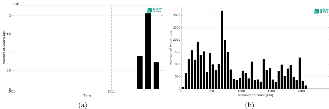
Figure 1: Number of match-ups between TSG (CSIC-UTM) and CCI SSS L4 Merged-OI v4.4 - 7-day running (ESA) SSS as a function of time (a) and as function of the distance to coast (b) over the Tropical Pacific Ocean Pi-MEP region and for the full satellite product period.
