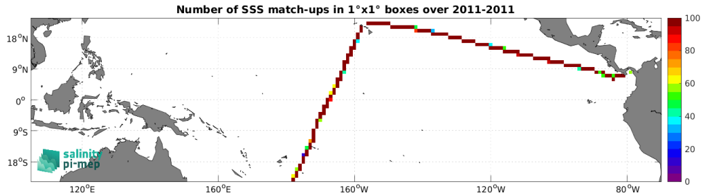
Figure 4: Number of SSS match-ups between TSG (CSIC-UTM) SSS and the CCI SSS L4 Merged-OI v4.4 - 7-day running (ESA) SSS product for the Tropical Pacific Ocean Pi-MEP region over 1^\circ \times 1^\circ boxes and for the full satellite product period.
