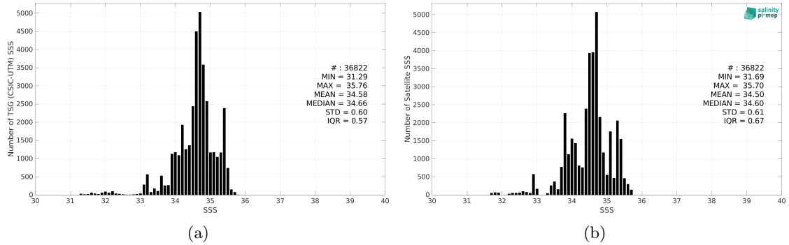
Figure 2: Histograms of SSS from TSG (CSIC-UTM) (a) and CCI SSS L4 Merged-OI v4.4 - 7-day running (ESA) (b) considering all match-up pairs per bins of 0.1 over the Tropical Pacific Ocean Pi-MEP region and for the full satellite product period.
