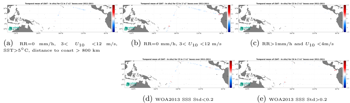
Figure 12: Temporal mean gridded over spatial boxes of size 1^\circ \times 1^\circ of \Delta SSS (CCI SSS L4 Merged-OI v4.4 - 7-day running (ESA) - TSG (CSIC-UTM)) for 5 different subdatasets corresponding to:RR=0 mm/h, 3 < U_{10} < 12 m/s, SST > 5^\circ\text{C} , distance to coast > 800 km (a), RR=0 mm/h, 3 < U_{10} < 12 m/s (b), RR > 1 mm/h and U_{10} < 4 m/s (c), WOA2013 SSS Std < 0.2 (d), WOA2013 SSS Std > 0.2 (e).
