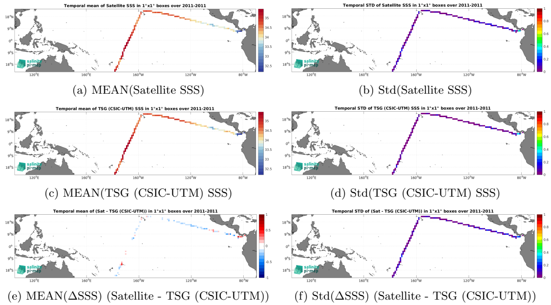
Figure 6: Temporal mean (left) and Std (right) of SSS from CCI SSS L4 Merged-OI v4.4 - 7-day running (ESA) (top), TSG (CSIC-UTM) (middle), and of \Delta SSS (Satellite - TSG (CSIC-UTM)). Only match-up pairs are used to generate these maps.
