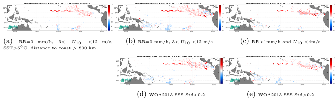
Figure 11: Temporal mean gridded over spatial boxes of size 1^\circ \times 1^\circ of \Delta SSS (CCI SSS L4 Merged-OI v4.4 - 7-day running (ESA) - Surface drifters) for 5 different subdatasets corresponding to: RR=0 mm/h, 3 < U_{10} < 12 m/s, SST > 5^\circ\text{C} , distance to coast > 800 km (a), RR=0 mm/h, 3 < U_{10} < 12 m/s (b), RR > 1 mm/h and U_{10} < 4 m/s (c), WOA2013 SSS Std < 0.2 (d), WOA2013 SSS Std > 0.2 (e).
