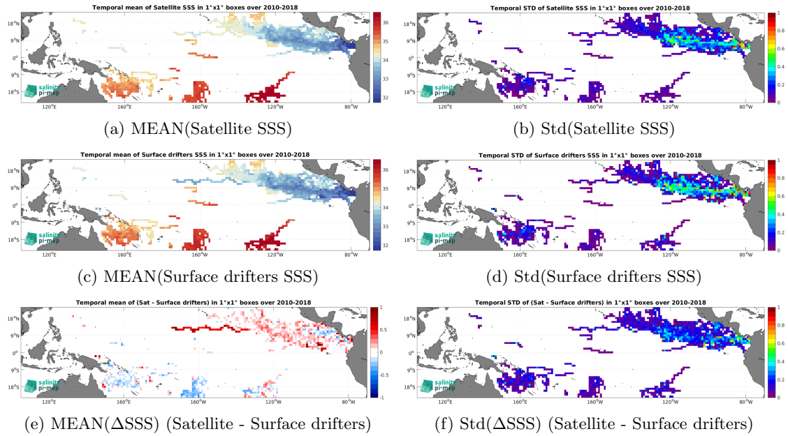
Figure 5: Temporal mean (left) and Std (right) of SSS from CCI SSS L4 Merged-OI v4.4 - 7-day running (ESA) (top), Surface drifters (middle), and of \Delta SSS (Satellite - Surface drifters). Only match-up pairs are used to generate these maps.
