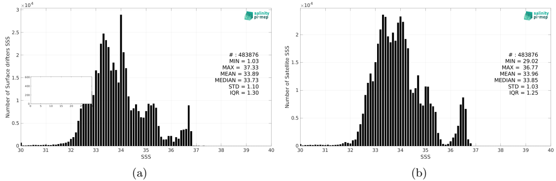
Figure 2: Histograms of SSS from Surface drifters (a) and CCI SSS L4 Merged-OI v4.4 - 7-day running (ESA) (b) considering all match-up pairs per bins of 0.1 over the Tropical Pacific Ocean Pi-MEP region and for the full satellite product period.
