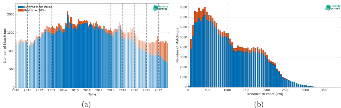
Figure 1: Number of match-ups between Argo and CCI SSS L4 Merged-OI v4.4 - 7-day running (ESA) SSS as a function of time (a) and as function of the distance to coast (b) over the Tropical Pacific Ocean Pi-MEP region and for the full satellite product period.
