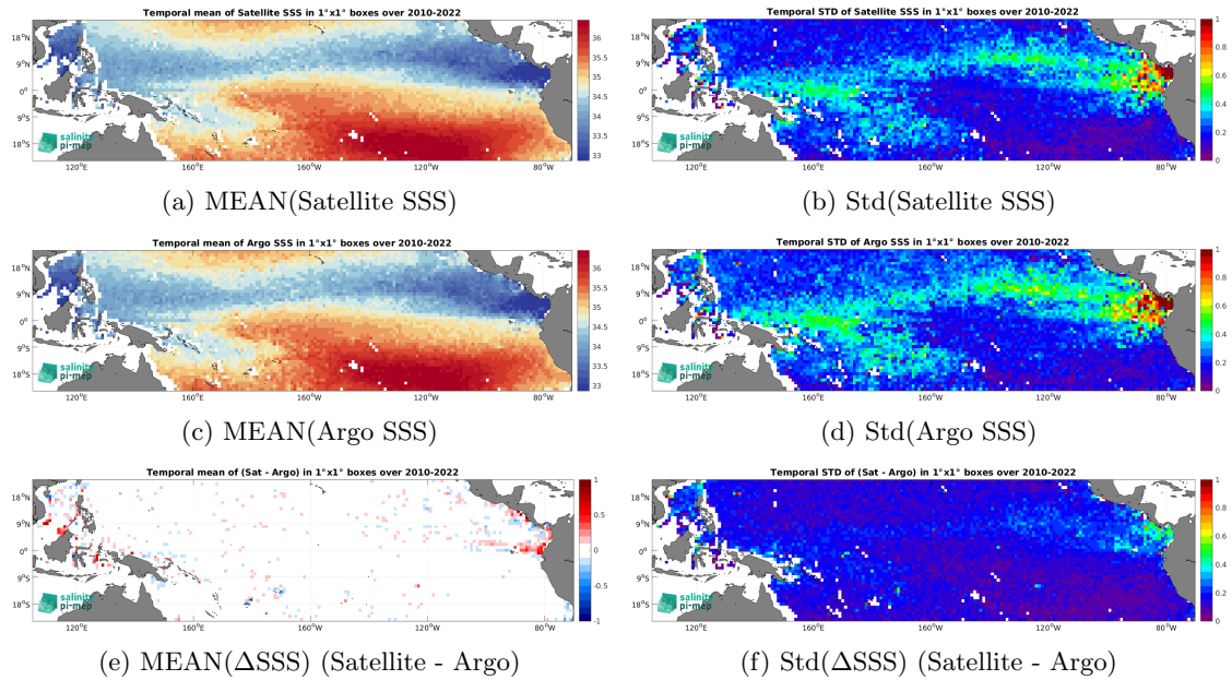
Figure 6: Temporal mean (left) and Std (right) of SSS from CCI SSS L4 Merged-OI v4.4 - 7-day running (ESA) (top), Argo (middle), and of \Delta SSS (Satellite - Argo). Only match-up pairs are used to generate these maps.
