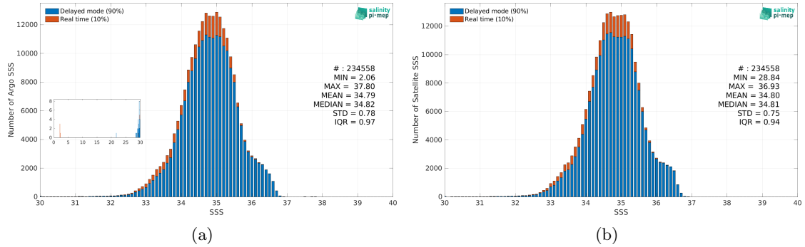
Figure 2: Histograms of SSS from Argo (a) and CCI SSS L4 Merged-OI v4.4 - 7-day running (ESA) (b) considering all match-up pairs per bins of 0.1 over the Tropical Pacific Ocean Pi-MEP region and for the full satellite product period.
