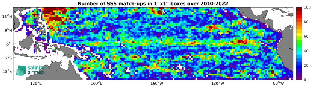
Figure 4: Number of SSS match-ups between Argo SSS and the CCI SSS L4 Merged-OI v4.4 - 7-day running (ESA) SSS product for the Tropical Pacific Ocean Pi-MEP region over 1^\circ \times 1^\circ boxes and for the full satellite product period.
