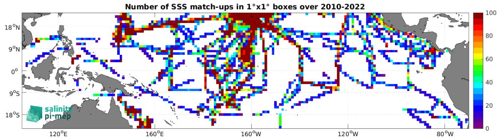
Figure 4: Number of SSS match-ups between TSG (SAMOS) SSS and the CCI SSS L4 Merged-OI v4.4 - 30-day running (ESA) SSS product for the Tropical Pacific Ocean Pi-MEP region over 1^\circ \times 1^\circ boxes and for the full satellite product period.
