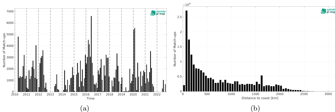
Figure 1: Number of match-ups between TSG (SAMOS) and CCI SSS L4 Merged-OI v4.4 - 30-day running (ESA) SSS as a function of time (a) and as function of the distance to coast (b) over the Tropical Pacific Ocean Pi-MEP region and for the full satellite product period.
