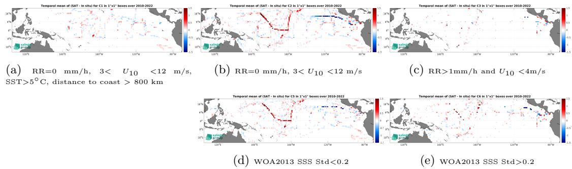
Figure 12: Temporal mean gridded over spatial boxes of size 1^\circ \times 1^\circ of \Delta SSS (CCI SSS L4 Merged-OI v4.4 - 30-day running (ESA) - TSG (SAMOS)) for 5 different subdatasets corresponding to: RR=0 mm/h, 3 < U_{10} < 12 m/s, SST > 5^\circ\text{C} , distance to coast > 800 km (a), RR=0 mm/h, 3 < U_{10} < 12 m/s (b), RR > 1 mm/h and U_{10} < 4 m/s (c), WOA2013 SSS Std < 0.2 (d), WOA2013 SSS Std > 0.2 (e).
