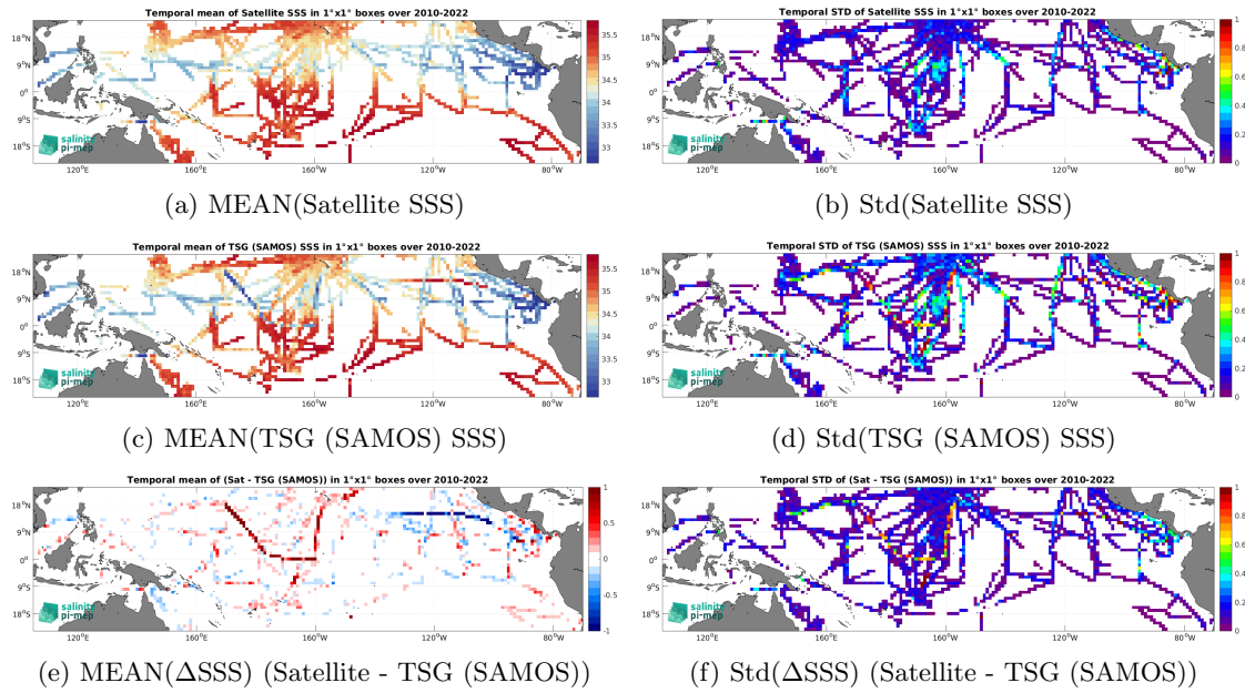
Figure 6: Temporal mean (left) and Std (right) of SSS from CCI SSS L4 Merged-OI v4.4 - 30-day running (ESA) (top), TSG (SAMOS) (middle), and of \Delta SSS (Satellite - TSG (SAMOS)). Only match-up pairs are used to generate these maps.
