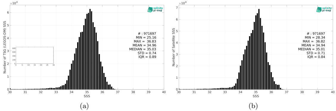
Figure 2: Histograms of SSS from TSG (LEGOS-DM) (a) and CCI SSS L4 Merged-OI v4.4 - 30-day running (ESA) (b) considering all match-up pairs per bins of 0.1 over the Tropical Pacific Ocean Pi-MEP region and for the full satellite product period.
