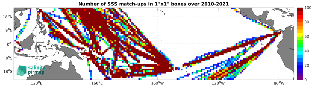
Figure 4: Number of SSS match-ups between TSG (LEGOS-DM) SSS and the CCI SSS L4 Merged-OI v4.4 - 30-day running (ESA) SSS product for the Tropical Pacific Ocean Pi-MEP region over 1^\circ \times 1^\circ boxes and for the full satellite product period.
