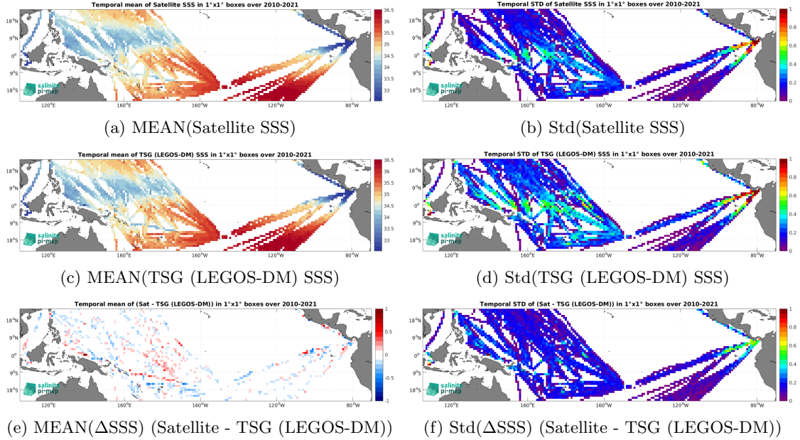
Figure 6: Temporal mean (left) and Std (right) of SSS from CCI SSS L4 Merged-OI v4.4 - 30-day running (ESA) (top), TSG (LEGOS-DM) (middle), and of \Delta SSS (Satellite - TSG (LEGOS-DM)). Only match-up pairs are used to generate these maps.
