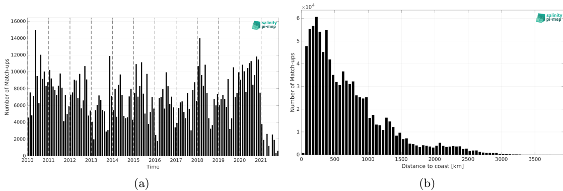
Figure 1: Number of match-ups between TSG (LEGOS-DM) and CCI SSS L4 Merged-OI v4.4 - 30-day running (ESA) SSS as a function of time (a) and as function of the distance to coast (b) over the Tropical Pacific Ocean Pi-MEP region and for the full satellite product period.
