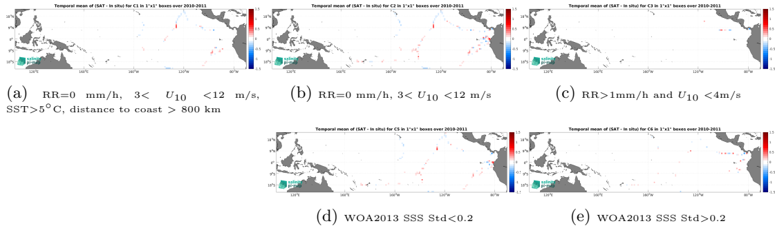
Figure 12: Temporal mean gridded over spatial boxes of size 1^{\circ}\times 1^{\circ} of \Delta SSS (CCI SSS L4 Merged-OI v4.4 - 30-day running (ESA) - TSG (GOSUD-Sailing-ship)) for 5 different subdatasets corresponding to:RR=0 mm/h, 3 < U_{10} < 12 m/s, SST >5^{\circ}\text{C} , distance to coast > 800 km (a), RR=0 mm/h, 3 < U_{10} < 12 m/s (b), RR >1 mm/h and U_{10} < 4 m/s (c), WOA2013 SSS Std <0.2 (d), WOA2013 SSS Std >0.2 (e).
