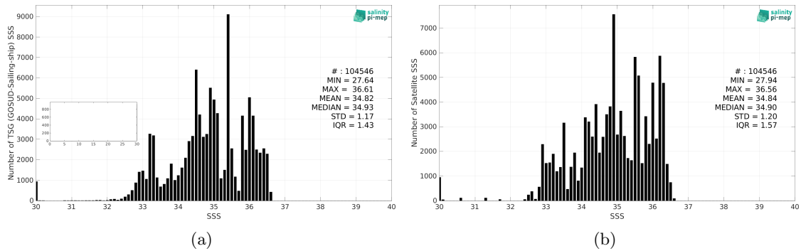
Figure 2: Histograms of SSS from TSG (GOSUD-Sailing-ship) (a) and CCI SSS L4 Merged-OI v4.4 - 30-day running (ESA) (b) considering all match-up pairs per bins of 0.1 over the Tropical Pacific Ocean Pi-MEP region and for the full satellite product period.
