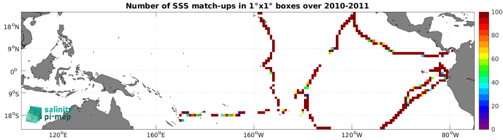
Figure 4: Number of SSS match-ups between TSG (GOSUD-Sailing-ship) SSS and the CCI SSS L4 Merged-OI v4.4 - 30-day running (ESA) SSS product for the Tropical Pacific Ocean Pi-MEP region over 1^\circ \times 1^\circ boxes and for the full satellite product period.
