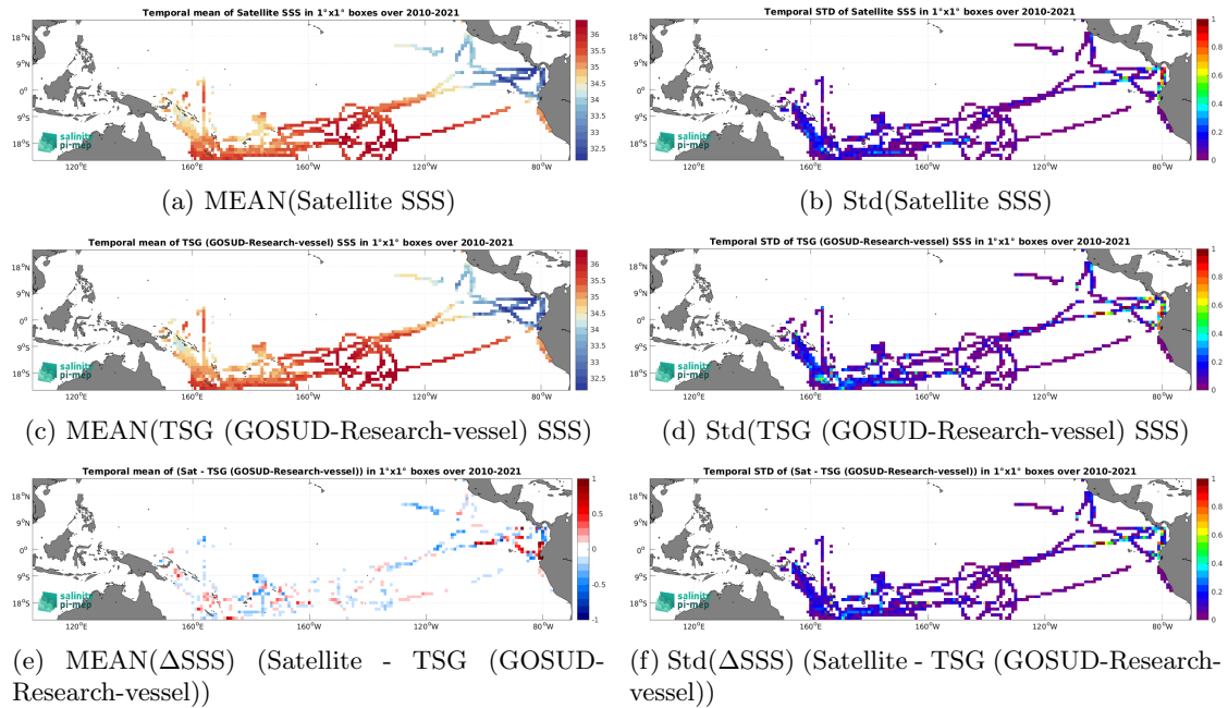
Figure 6: Temporal mean (left) and Std (right) of SSS from CCI SSS L4 Merged-OI v4.4 - 30-day running (ESA) (top), TSG (GOSUD-Research-vessel) (middle), and of \Delta SSS (Satellite - TSG (GOSUD-Research-vessel)). Only match-up pairs are used to generate these maps.
