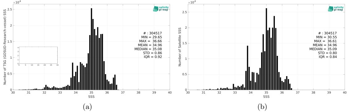
Figure 2: Histograms of SSS from TSG (GOSUD-Research-vessel) (a) and CCI SSS L4 Merged-OI v4.4 - 30-day running (ESA) (b) considering all match-up pairs per bins of 0.1 over the Tropical Pacific Ocean Pi-MEP region and for the full satellite product period.
