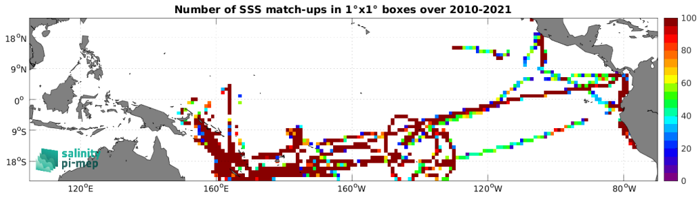
Figure 4: Number of SSS match-ups between TSG (GOSUD-Research-vessel) SSS and the CCI SSS L4 Merged-OI v4.4 - 30-day running (ESA) SSS product for the Tropical Pacific Ocean Pi-MEP region over 1^\circ \times 1^\circ boxes and for the full satellite product period.
