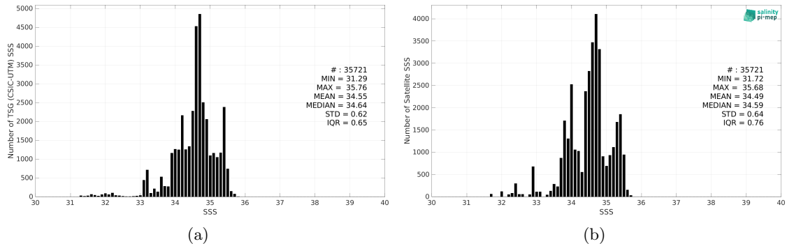
Figure 2: Histograms of SSS from TSG (CSIC-UTM) (a) and CCI SSS L4 Merged-OI v4.4 - 30-day running (ESA) (b) considering all match-up pairs per bins of 0.1 over the Tropical Pacific Ocean Pi-MEP region and for the full satellite product period.
