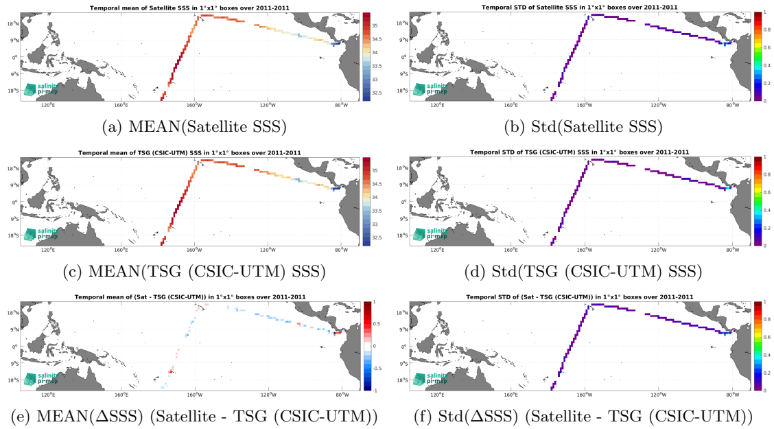
Figure 6: Temporal mean (left) and Std (right) of SSS from CCI SSS L4 Merged-OI v4.4 - 30-day running (ESA) (top), TSG (CSIC-UTM) ( in situ ) dataset (middle), and of \Delta SSS (Satellite - TSG (CSIC-UTM)). Only match-up pairs are used to generate these maps.
