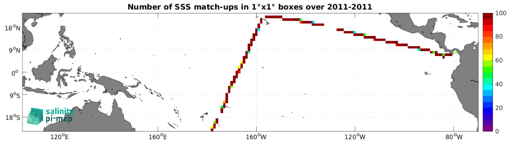
Figure 4: Number of SSS match-ups between TSG (CSIC-UTM) SSS and the CCI SSS L4 Merged-OI v4.4 - 30-day running (ESA) SSS product for the Tropical Pacific Ocean Pi-MEP region over 1^\circ \times 1^\circ boxes and for the full satellite product period.
