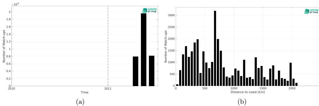
Figure 1: Number of match-ups between TSG (CSIC-UTM) and CCI SSS L4 Merged-OI v4.4 - 30-day running (ESA) SSS as a function of time (a) and as function of the distance to coast (b) over the Tropical Pacific Ocean Pi-MEP region and for the full satellite product period.
