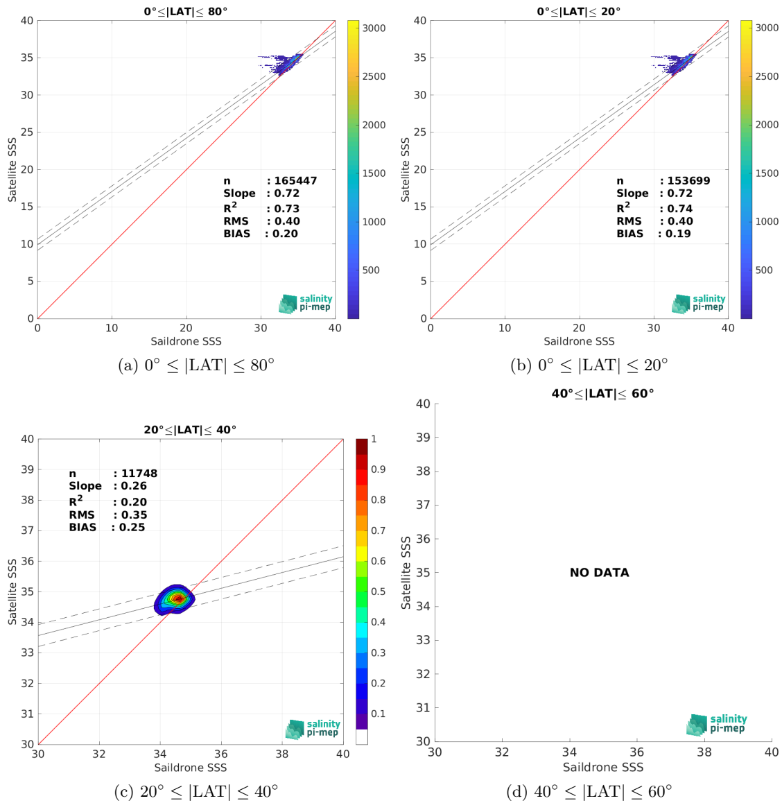
Figure 9: Contour maps of the concentration of CCI SSS L4 Merged-OI v4.4 - 30-day running (ESA) SSS (y-axis) versus Saildrone SSS (x-axis) at match-up pairs for different latitude bands. For each plot, the red line shows x=y . The black thin and dashed lines indicate a linear fit through the data cloud and the \pm 95\% confidence levels, respectively. The number match-up pairs n , the slope and R^2 coefficient of the linear fit, the root mean square (RMS) and the mean bias between satellite and in situ data are indicated for each latitude band in each plots.
