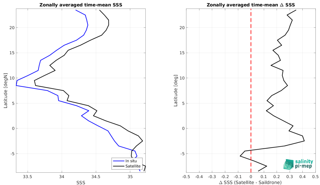
Figure 8: Left panel: Zonal mean SSS from CCI SSS L4 Merged-OI v4.4 - 30-day running (ESA) satellite product (black) and from Sairdron (blue). Right panel: Zonal mean of \Delta SSS (Satellite - Sairdron) for all the collected Pi-MEP match-up pairs estimated over the full satellite product period.
