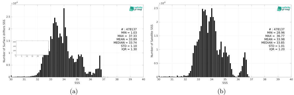
Figure 2: Histograms of SSS from Surface drifters (a) and CCI SSS L4 Merged-OI v4.4 - 30-day running (ESA) (b) considering all match-up pairs per bins of 0.1 over the Tropical Pacific Ocean Pi-MEP region and for the full satellite product period.
