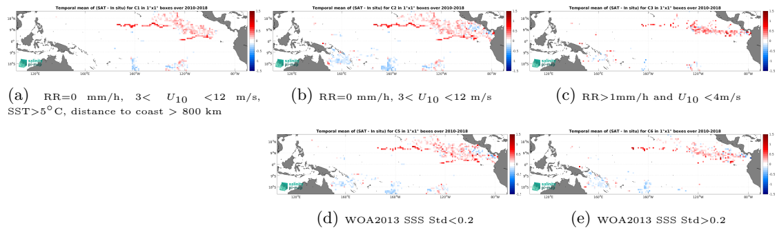
Figure 11: Temporal mean gridded over spatial boxes of size 1^\circ \times 1^\circ of \Delta\text{SSS} (CCI SSS L4 Merged-OI v4.4 - 30-day running (ESA) - Surface drifters) for 5 different subdatasets corresponding to: RR=0 mm/h, 3 < U_{10} < 12 m/s, SST > 5^\circ\text{C} , distance to coast > 800 km (a), RR=0 mm/h, 3 < U_{10} < 12 m/s (b), RR > 1 mm/h and U_{10} < 4 m/s (c), WOA2013 SSS Std < 0.2 (d), WOA2013 SSS Std > 0.2 (e).
