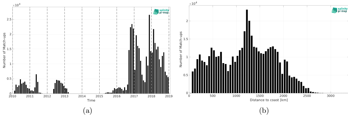
Figure 1: Number of match-ups between Surface drifters and CCI SSS L4 Merged-OI v4.4 - 30-day running (ESA) SSS as a function of time (a) and as function of the distance to coast (b) over the Tropical Pacific Ocean Pi-MEP region and for the full satellite product period.
