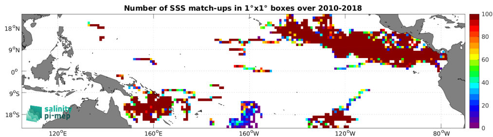
Figure 3: Number of SSS match-ups between Surface drifters SSS and the CCI SSS L4 Merged-OI v4.4 - 30-day running (ESA) SSS product for the Tropical Pacific Ocean Pi-MEP region over 1^\circ \times 1^\circ boxes and for the full satellite product period.
