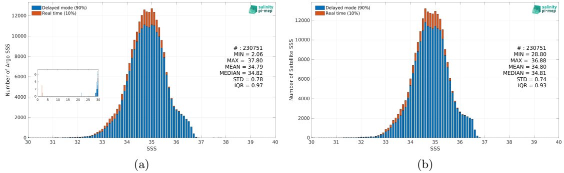
Figure 2: Histograms of SSS from Argo (a) and CCI SSS L4 Merged-OI v4.4 - 30-day running (ESA) (b) considering all match-up pairs per bins of 0.1 over the Tropical Pacific Ocean Pi-MEP region and for the full satellite product period.
