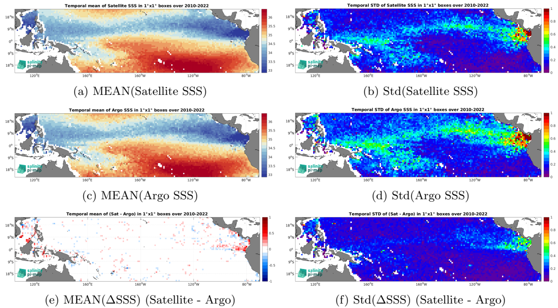
Figure 6: Temporal mean (left) and Std (right) of SSS from CCI SSS L4 Merged-OI v4.4 - 30-day running (ESA) (top), Argo (middle), and of \Delta SSS (Satellite - Argo). Only match-up pairs are used to generate these maps.
