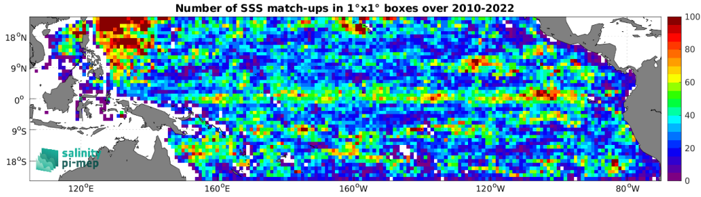
Figure 4: Number of SSS match-ups between Argo SSS and the CCI SSS L4 Merged-OI v4.4 - 30-day running (ESA) SSS product for the Tropical Pacific Ocean Pi-MEP region over 1^\circ \times 1^\circ boxes and for the full satellite product period.
