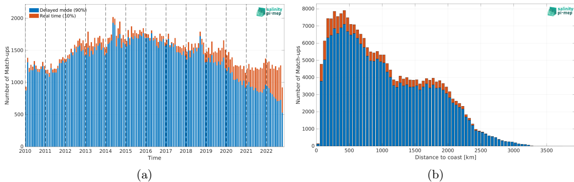
Figure 1: Number of match-ups between Argo and CCI SSS L4 Merged-OI v4.4 - 30-day running (ESA) SSS as a function of time (a) and as function of the distance to coast (b) over the Tropical Pacific Ocean Pi-MEP region and for the full satellite product period.
