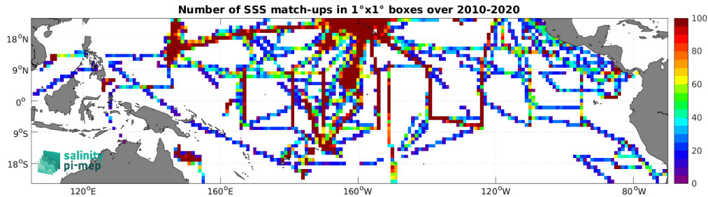
Figure 4: Number of SSS match-ups between TSG (SAMOS) SSS and the CCI SSS L4 Merged-OI v3.2 - 7-day running (ESA) SSS product for the Tropical Pacific Ocean Pi-MEP region over 1^\circ \times 1^\circ boxes and for the full satellite product period.
