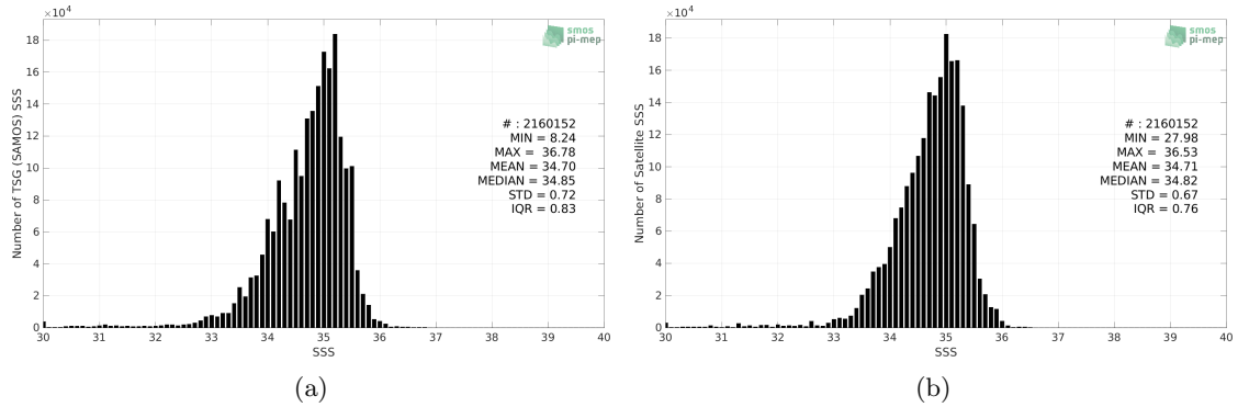
Figure 2: Histograms of SSS from TSG (SAMOS) (a) and CCI SSS L4 Merged-OI v3.2 - 7-day running (ESA) (b) considering all match-up pairs per bins of 0.1 over the Tropical Pacific Ocean Pi-MEP region and for the full satellite product period.
