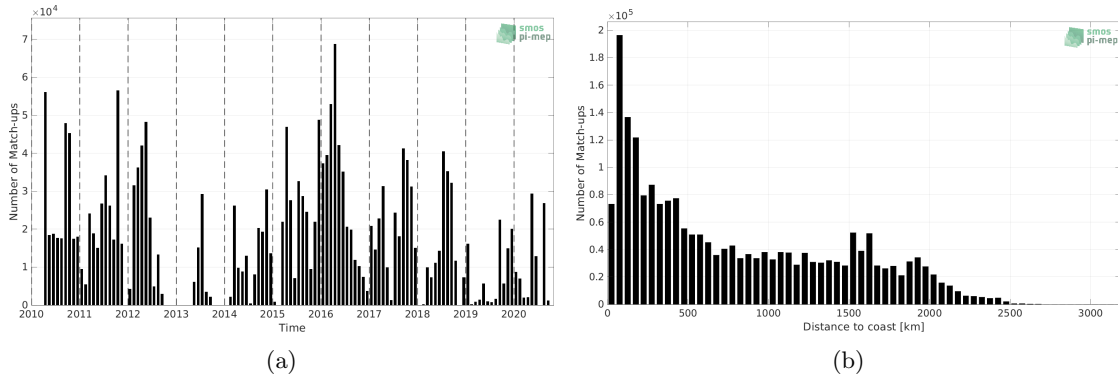
Figure 1: Number of match-ups between TSG (SAMOS) and CCI SSS L4 Merged-OI v3.2 - 7-day running (ESA) SSS as a function of time (a) and as function of the distance to coast (b) over the Tropical Pacific Ocean Pi-MEP region and for the full satellite product period.
