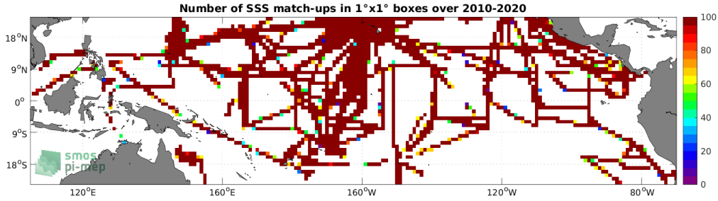
Figure 4: Number of SSS match-ups between TSG (SAMOS) SSS and the CCI SSS L4 Merged-OI v3.2 - 7-day running (ESA) SSS product for the Tropical Pacific Ocean Pi-MEP region over 1^\circ \times 1^\circ boxes and for the full satellite product period.
