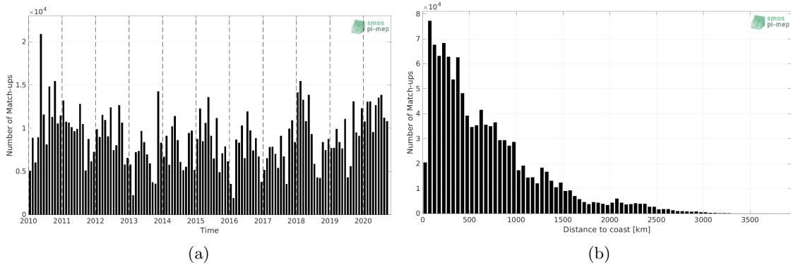
Figure 1: Number of match-ups between TSG (LEGOS-DM) and CCI SSS L4 Merged-OI v3.2 - 7-day running (ESA) SSS as a function of time (a) and as function of the distance to coast (b) over the Tropical Pacific Ocean Pi-MEP region and for the full satellite product period.
