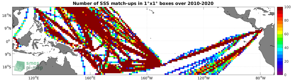
Figure 4: Number of SSS match-ups between TSG (LEGOS-DM) SSS and the CCI SSS L4 Merged-OI v3.2 - 7-day running (ESA) SSS product for the Tropical Pacific Ocean Pi-MEP region over 1^\circ \times 1^\circ boxes and for the full satellite product period.
