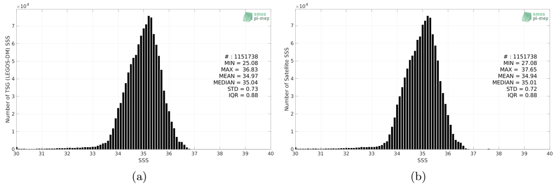
Figure 2: Histograms of SSS from TSG (LEGOS-DM) (a) and CCI SSS L4 Merged-OI v3.2 - 7-day running (ESA) (b) considering all match-up pairs per bins of 0.1 over the Tropical Pacific Ocean Pi-MEP region and for the full satellite product period.
