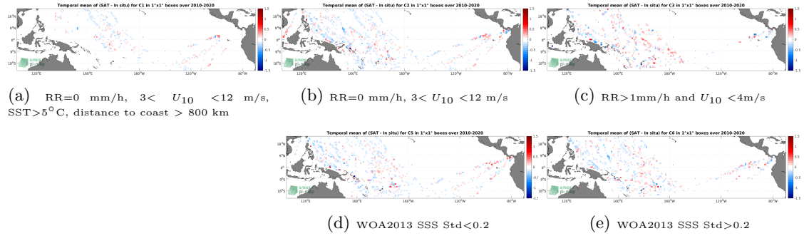
Figure 12: Temporal mean gridded over spatial boxes of size 1^{\circ}\times 1^{\circ} of \Delta\text{SSS} (CCI SSS L4 Merged-OI v3.2 - 7-day running (ESA) - TSG (LEGOS-DM)) for 5 different subdatasets corresponding to:RR=0 mm/h, 3 < U_{10} < 12 m/s, SST >5^{\circ}\text{C} , distance to coast > 800 km (a), RR=0 mm/h, 3 < U_{10} < 12 m/s (b), RR >1 mm/h and U_{10} < 4 m/s (c), WOA2013 SSS Std <0.2 (d), WOA2013 SSS Std >0.2 (e).
