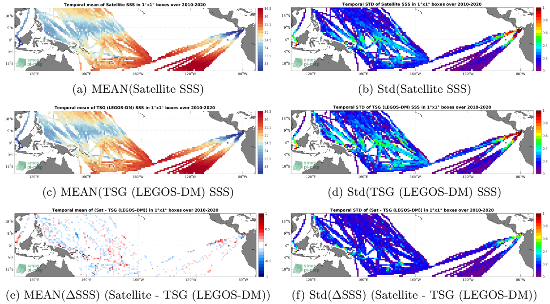
Figure 6: Temporal mean (left) and Std (right) of SSS from CCI SSS L4 Merged-OI v3.2 - 7-day running (ESA) (top), TSG (LEGOS-DM) (middle), and of \Delta SSS (Satellite - TSG (LEGOS-DM)). Only match-up pairs are used to generate these maps.
