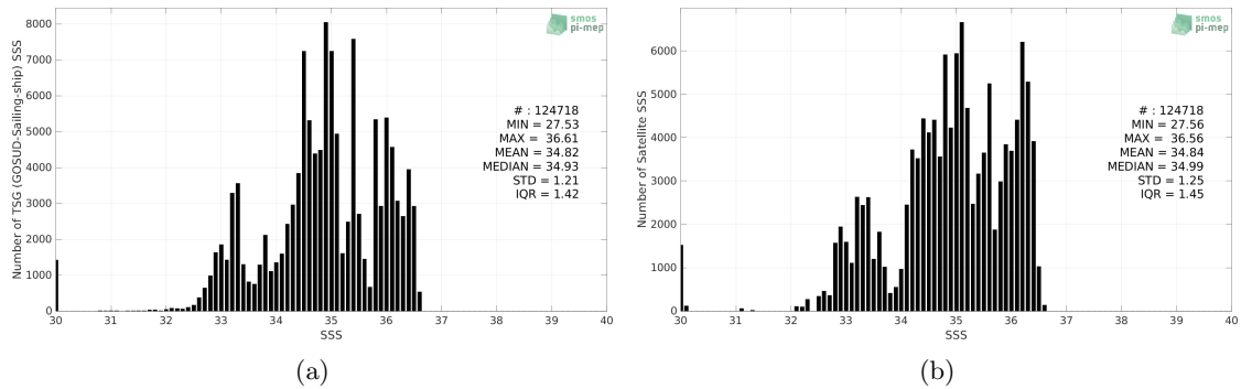
Figure 2: Histograms of SSS from TSG (GOSUD-Sailing-ship) (a) and CCI SSS L4 Merged-OI v3.2 - 7-day running (ESA) (b) considering all match-up pairs per bins of 0.1 over the Tropical Pacific Ocean Pi-MEP region and for the full satellite product period.
