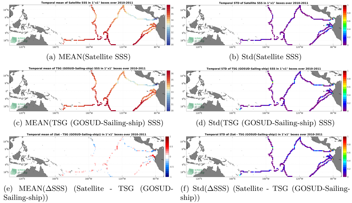
Figure 6: Temporal mean (left) and Std (right) of SSS from CCI SSS L4 Merged-OI v3.2 - 7-day running (ESA) (top), TSG (GOSUD-Sailing-ship) (middle), and of \Delta SSS (Satellite - TSG (GOSUD-Sailing-ship)). Only match-up pairs are used to generate these maps.
