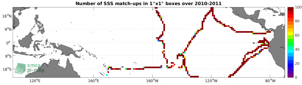
Figure 4: Number of SSS match-ups between TSG (GOSUD-Sailing-ship) SSS and the CCI SSS L4 Merged-OI v3.2 - 7-day running (ESA) SSS product for the Tropical Pacific Ocean Pi-MEP region over 1^\circ \times 1^\circ boxes and for the full satellite product period.
