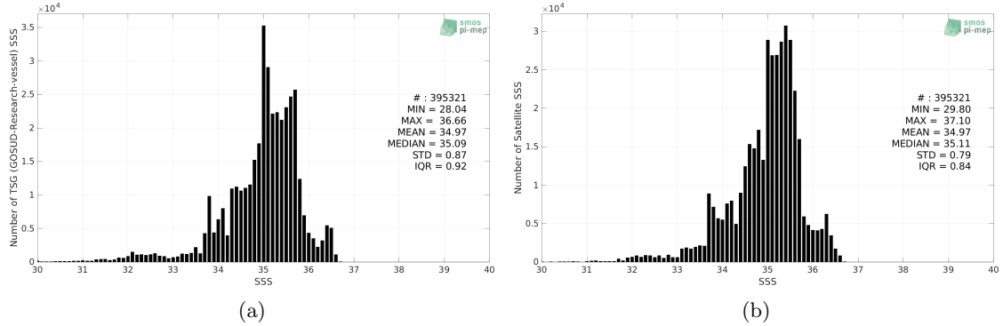
Figure 2: Histograms of SSS from TSG (GOSUD-Research-vessel) (a) and CCI SSS L4 Merged-OI v3.2 - 7-day running (ESA) (b) considering all match-up pairs per bins of 0.1 over the Tropical Pacific Ocean Pi-MEP region and for the full satellite product period.
