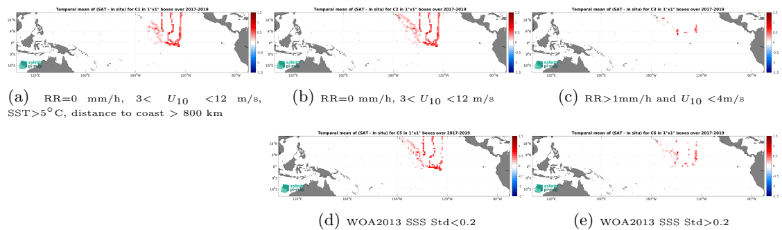
Figure 12: Temporal mean gridded over spatial boxes of size 1^\circ \times 1^\circ of \Delta SSS (CCI SSS L4 Merged-OI v3.2 - 7-day running (ESA) - Sailydrone) for 5 different subdatasets corresponding to: RR=0 mm/h, 3 < U_{10} < 12 m/s, SST > 5^\circ\text{C} , distance to coast > 800 km (a), RR=0 mm/h, 3 < U_{10} < 12 m/s (b), RR > 1 mm/h and U_{10} < 4 m/s (c), WOA2013 SSS Std < 0.2 (d), WOA2013 SSS Std > 0.2 (e).
