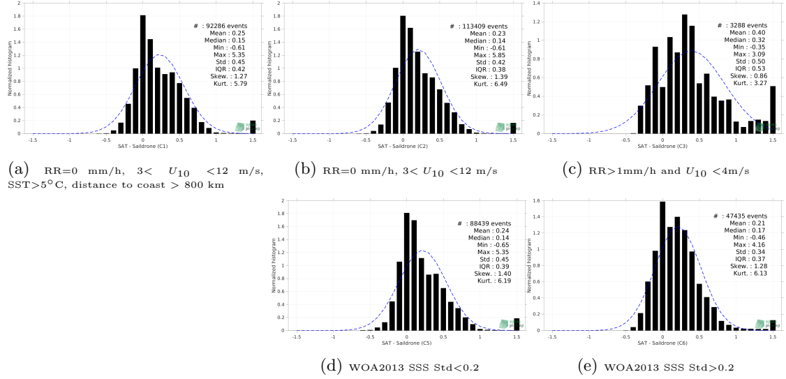
Figure 13: Normalized histogram of \Delta SSS (CCI SSS L4 Merged-OI v3.2 - 7-day running (ESA) - Saildrone) for 5 different subdatasets corresponding to: RR=0 mm/h, 3 < U_{10} < 12 m/s, SST>5°C, distance to coast > 800 km (a), RR=0 mm/h, 3 < U_{10} < 12 m/s (b), RR>1mm/h and U_{10} < 4 m/s (c), WOA2013 SSS Std<0.2 (d), WOA2013 SSS Std>0.2 (e).
