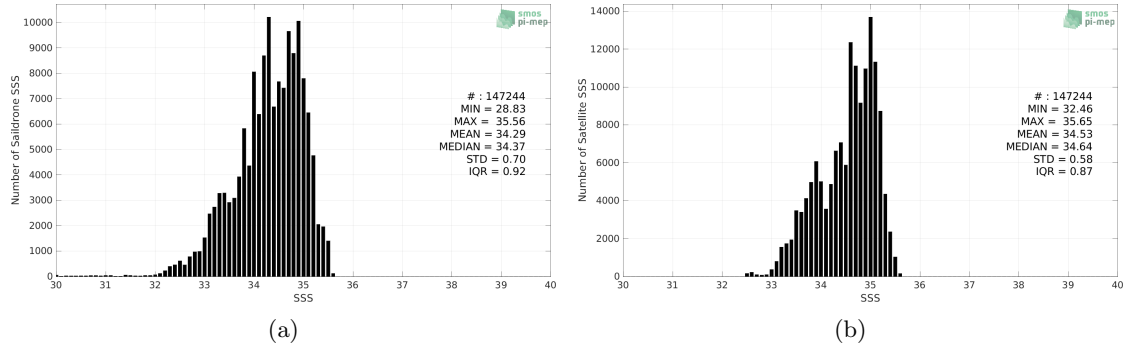
Figure 2: Histograms of SSS from Saildrone (a) and CCI SSS L4 Merged-OI v3.2 - 7-day running (ESA) (b) considering all match-up pairs per bins of 0.1 over the Tropical Pacific Ocean Pi-MEP region and for the full satellite product period.
