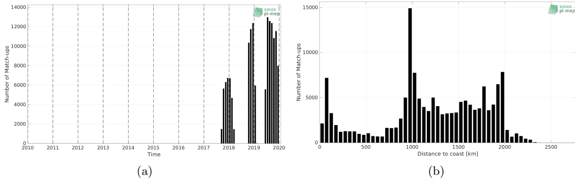
Figure 1: Number of match-ups between Saildrone and CCI SSS L4 Merged-OI v3.2 - 7-day running (ESA) SSS as a function of time (a) and as function of the distance to coast (b) over the Tropical Pacific Ocean Pi-MEP region and for the full satellite product period.
