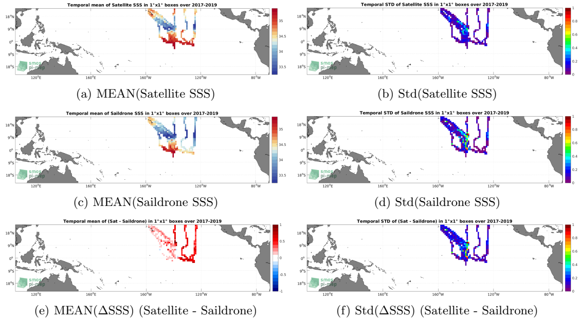
Figure 6: Temporal mean (left) and Std (right) of SSS from CCI SSS L4 Merged-OI v3.2 - 7-day running (ESA) (top), Saildrone (middle), and of \Delta SSS (Satellite - Saildrone). Only match-up pairs are used to generate these maps.
