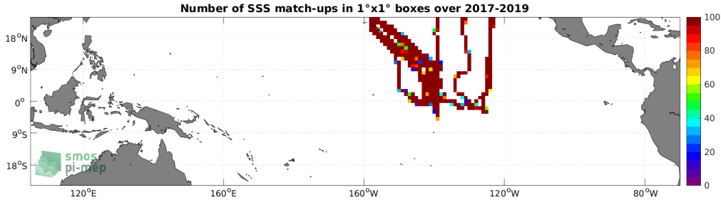
Figure 4: Number of SSS match-ups between Saildrone SSS and the CCI SSS L4 Merged-OI v3.2 - 7-day running (ESA) SSS product for the Tropical Pacific Ocean Pi-MEP region over 1^\circ \times 1^\circ boxes and for the full satellite product period.
