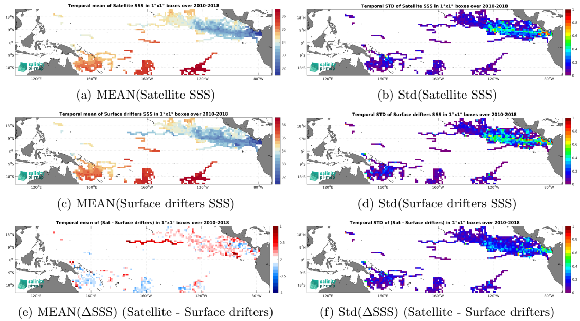
Figure 5: Temporal mean (left) and Std (right) of SSS from CCI SSS L4 Merged-OI v3.2 - 7-day running (ESA) (top), Surface drifters (middle), and of \Delta SSS (Satellite - Surface drifters). Only match-up pairs are used to generate these maps.
