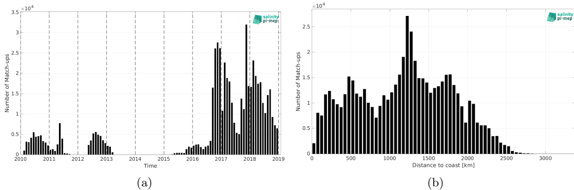
Figure 1: Number of match-ups between Surface drifters and CCI SSS L4 Merged-OI v3.2 - 7-day running (ESA) SSS as a function of time (a) and as function of the distance to coast (b) over the Tropical Pacific Ocean Pi-MEP region and for the full satellite product period.
