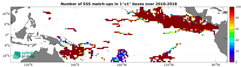
Figure 3: Number of SSS match-ups between Surface drifters SSS and the CCI SSS L4 Merged-OI v3.2 - 7-day running (ESA) SSS product for the Tropical Pacific Ocean Pi-MEP region over 1^\circ \times 1^\circ boxes and for the full satellite product period.
