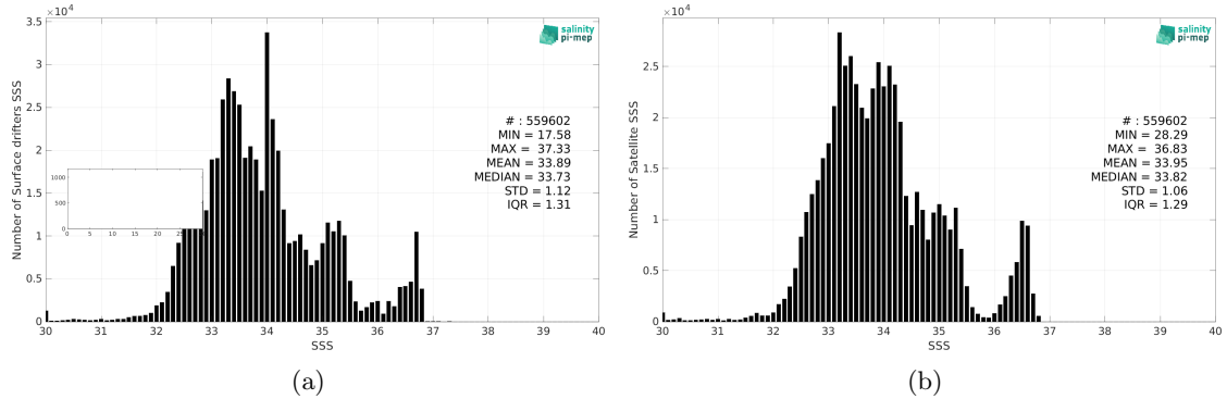
Figure 2: Histograms of SSS from Surface drifters (a) and CCI SSS L4 Merged-OI v3.2 - 7-day running (ESA) (b) considering all match-up pairs per bins of 0.1 over the Tropical Pacific Ocean Pi-MEP region and for the full satellite product period.
