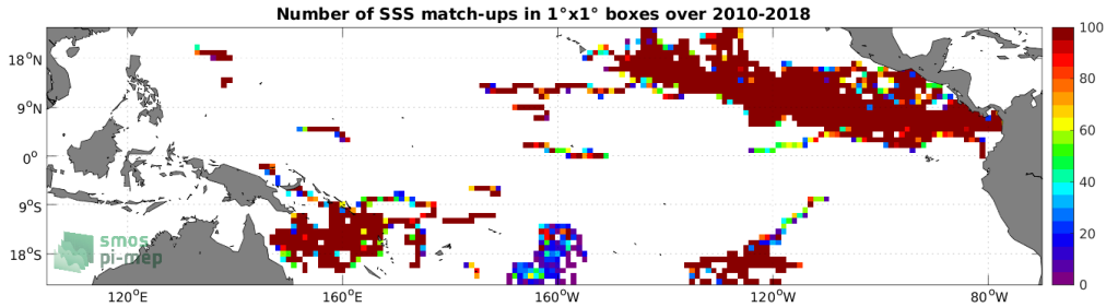
Figure 3: Number of SSS match-ups between Surface drifters SSS and the CCI SSS L4 Merged-OI v3.2 - 7-day running (ESA) SSS product for the Tropical Pacific Ocean Pi-MEP region over 1^\circ \times 1^\circ boxes and for the full satellite product period.
