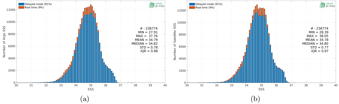
Figure 2: Histograms of SSS from Argo (a) and CCI SSS L4 Merged-OI v3.2 - 7-day running (ESA) (b) considering all match-up pairs per bins of 0.1 over the Tropical Pacific Ocean Pi-MEP region and for the full satellite product period.
