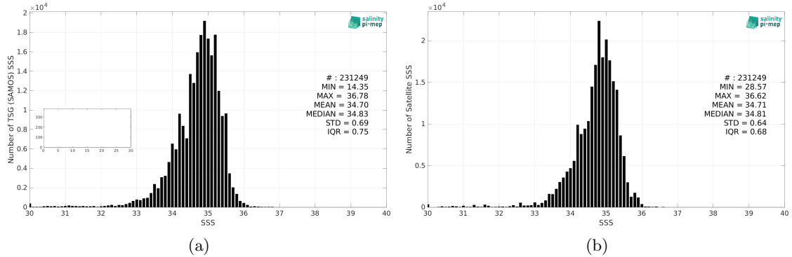
Figure 2: Histograms of SSS from TSG (SAMOS) (a) and CCI SSS L4 Merged-OI v3.2 - 30-day running (ESA) (b) considering all match-up pairs per bins of 0.1 over the Tropical Pacific Ocean Pi-MEP region and for the full satellite product period.
