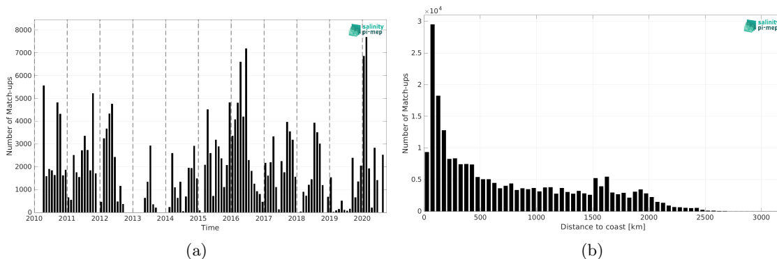
Figure 1: Number of match-ups between TSG (SAMOS) and CCI SSS L4 Merged-OI v3.2 - 30-day running (ESA) SSS as a function of time (a) and as function of the distance to coast (b) over the Tropical Pacific Ocean Pi-MEP region and for the full satellite product period.
