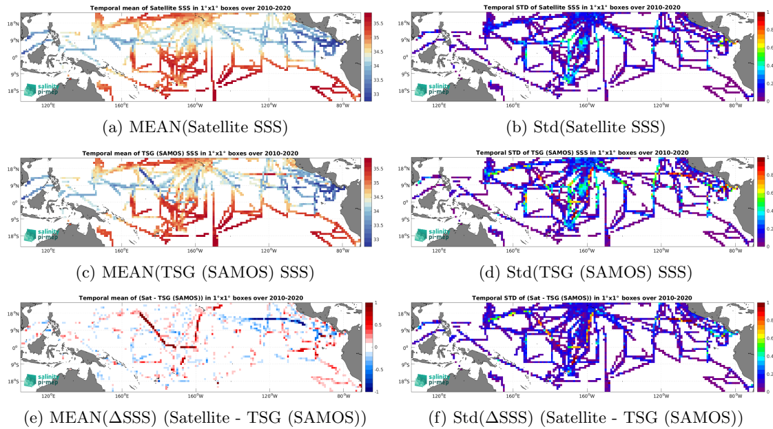
Figure 6: Temporal mean (left) and Std (right) of SSS from CCI SSS L4 Merged-OI v3.2 - 30-day running (ESA) (top), TSG (SAMOS) (middle), and of \Delta SSS (Satellite - TSG (SAMOS)). Only match-up pairs are used to generate these maps.
