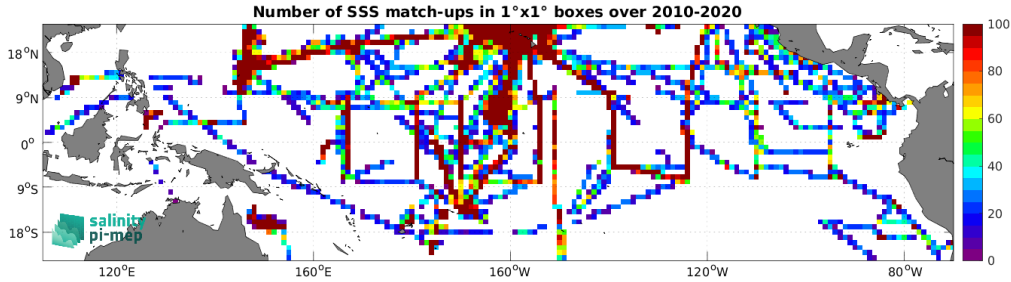
Figure 4: Number of SSS match-ups between TSG (SAMOS) SSS and the CCI SSS L4 Merged-OI v3.2 - 30-day running (ESA) SSS product for the Tropical Pacific Ocean Pi-MEP region over 1^\circ \times 1^\circ boxes and for the full satellite product period.
