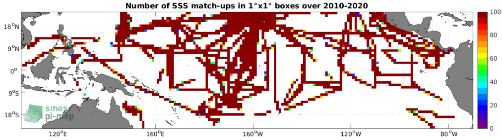
Figure 4: Number of SSS match-ups between TSG (SAMOS) SSS and the CCI SSS L4 Merged-OI v3.2 - 30-day running (ESA) SSS product for the Tropical Pacific Ocean Pi-MEP region over 1^\circ \times 1^\circ boxes and for the full satellite product period.
