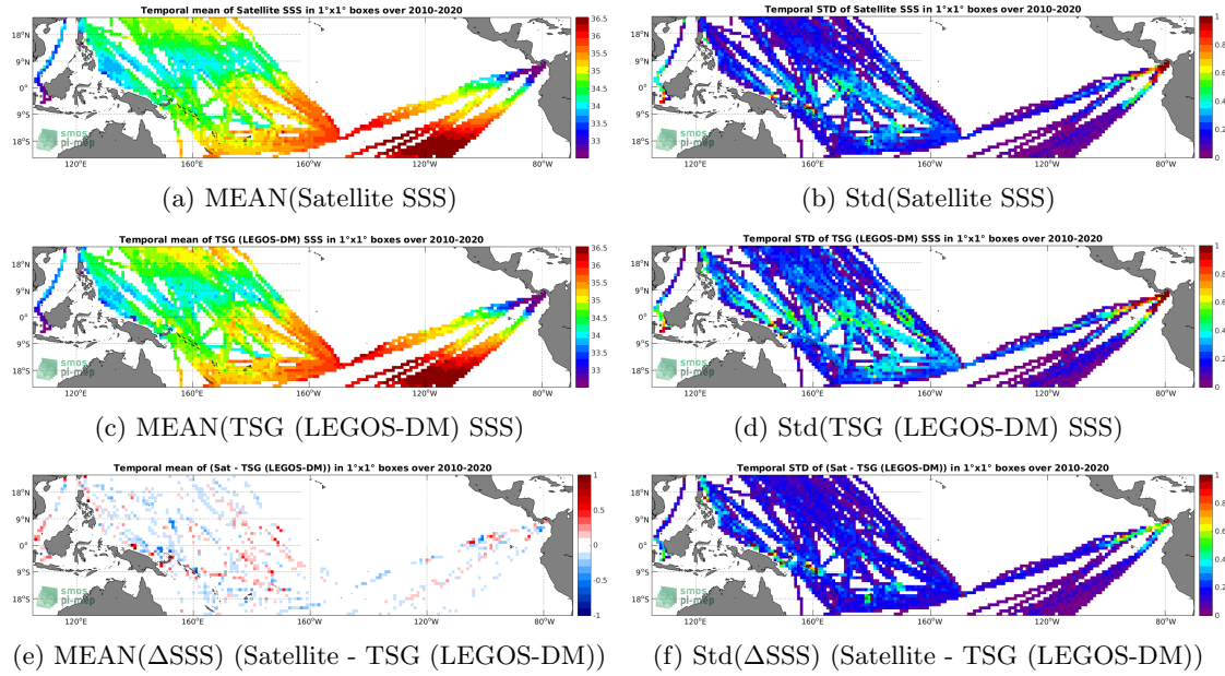
Figure 6: Temporal mean (left) and Std (right) of SSS from CCI SSS L4 Merged-OI v3.2 - 30-day running (ESA) (top), TSG (LEGOS-DM) (middle), and of \Delta SSS (Satellite - TSG (LEGOS-DM)). Only match-up pairs are used to generate these maps.
