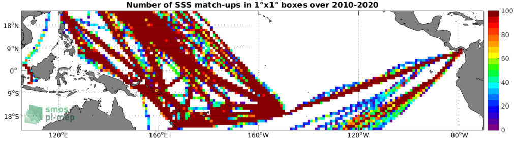
Figure 4: Number of SSS match-ups between TSG (LEGOS-DM) SSS and the CCI SSS L4 Merged-OI v3.2 - 30-day running (ESA) SSS product for the Tropical Pacific Ocean Pi-MEP region over 1^\circ \times 1^\circ boxes and for the full satellite product period.
