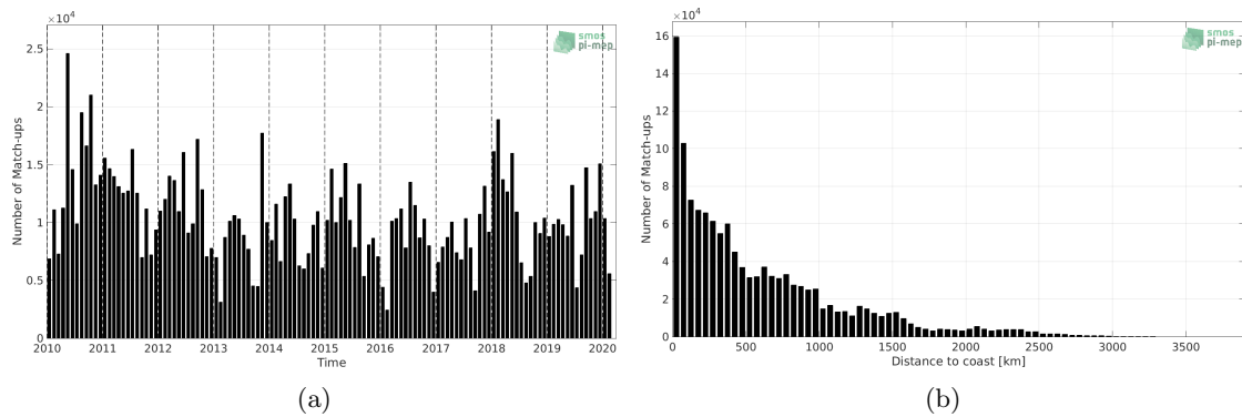
Figure 1: Number of match-ups between TSG (LEGOS-DM) and CCI SSS L4 Merged-OI v3.2 - 30-day running (ESA) SSS as a function of time (a) and as function of the distance to coast (b) over the Tropical Pacific Ocean Pi-MEP region and for the full satellite product period.
