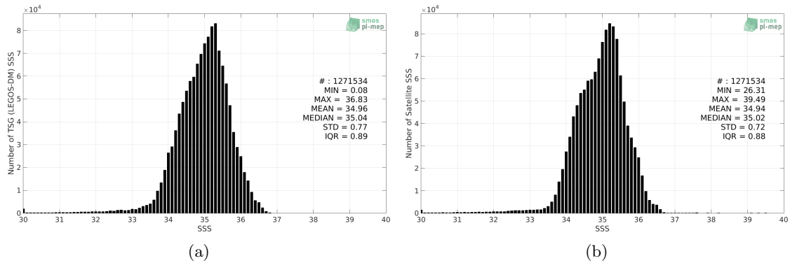
Figure 2: Histograms of SSS from TSG (LEGOS-DM) (a) and CCI SSS L4 Merged-OI v3.2 - 30-day running (ESA) (b) considering all match-up pairs per bins of 0.1 over the Tropical Pacific Ocean Pi-MEP region and for the full satellite product period.
