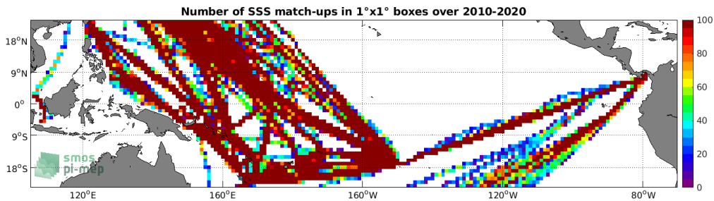
Figure 4: Number of SSS match-ups between TSG (LEGOS-DM) SSS and the CCI SSS L4 Merged-OI v3.2 - 30-day running (ESA) SSS product for the Tropical Pacific Ocean Pi-MEP region over 1°x1° boxes and for the full satellite product period.
