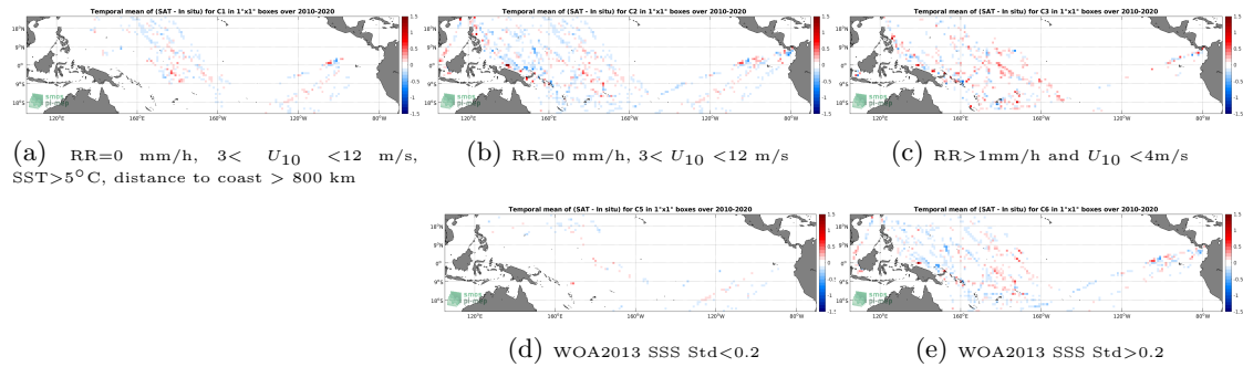
Figure 12: Temporal mean gridded over spatial boxes of size 1^{\circ}\times 1^{\circ} of \Delta\text{SSS} (CCI SSS L4 Merged-OI v3.2 - 30-day running (ESA) - TSG (LEGOS-DM)) for 5 different subdatasets corresponding to:RR=0 mm/h, 3 < U_{10} < 12 m/s, SST > 5^{\circ}\text{C} , distance to coast > 800 km (a), RR=0 mm/h, 3 < U_{10} < 12 m/s (b), RR > 1 mm/h and U_{10} < 4 m/s (c), WOA2013 SSS Std < 0.2 (d), WOA2013 SSS Std > 0.2 (e).
