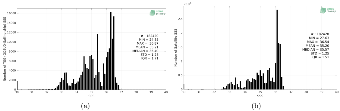
Figure 2: Histograms of SSS from TSG (GOSUD-Sailing-ship) (a) and CCI SSS L4 Merged-OI v3.2 - 30-day running (ESA) (b) considering all match-up pairs per bins of 0.1 over the Tropical Pacific Ocean Pi-MEP region and for the full satellite product period.
