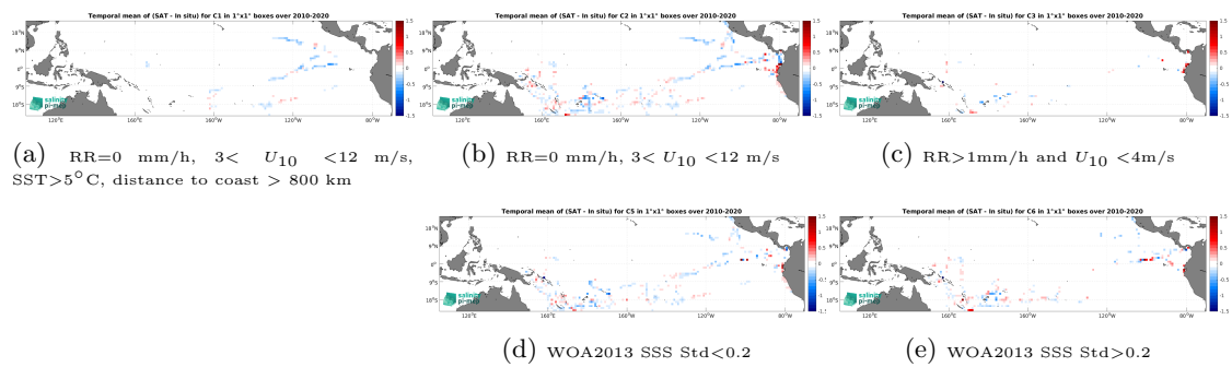
Figure 12: Temporal mean gridded over spatial boxes of size 1^\circ \times 1^\circ of \Delta\text{SSS} (CCI SSS L4 Merged-OI v3.2 - 30-day running (ESA) - TSG (GOSUD-Research-vessel)) for 5 different subdatasets corresponding to: RR=0 mm/h, 3 < U_{10} < 12 m/s, SST > 5°C, distance to coast > 800 km (a), RR=0 mm/h, 3 < U_{10} < 12 m/s (b), RR > 1mm/h and U_{10} < 4 m/s (c), WOA2013 SSS Std < 0.2 (d), WOA2013 SSS Std > 0.2 (e).
