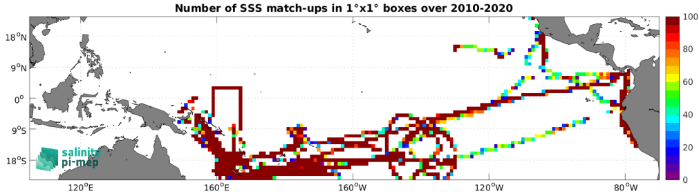
Figure 4: Number of SSS match-ups between TSG (GOSUD-Research-vessel) SSS and the CCI SSS L4 Merged-OI v3.2 - 30-day running (ESA) SSS product for the Tropical Pacific Ocean Pi-MEP region over 1^\circ \times 1^\circ boxes and for the full satellite product period.
