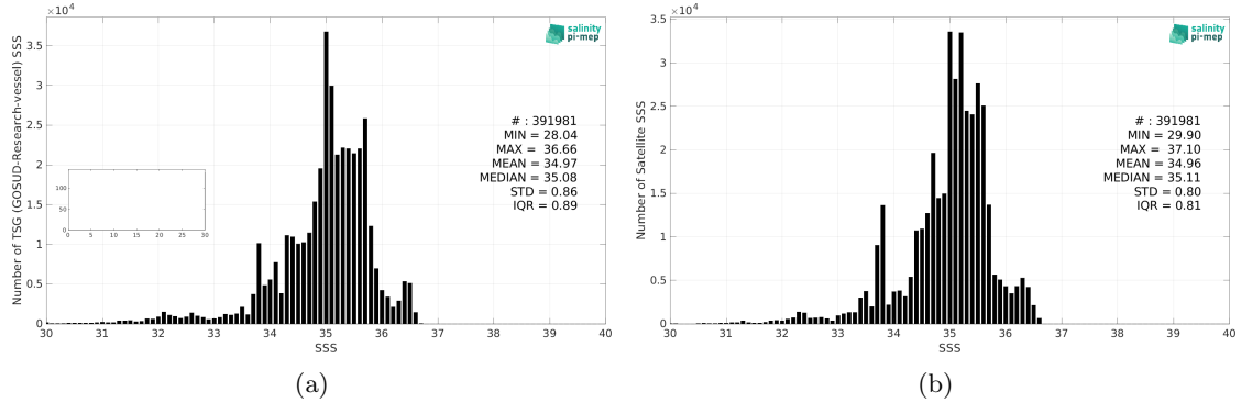
Figure 2: Histograms of SSS from TSG (GOSUD-Research-vessel) (a) and CCI SSS L4 Merged-OI v3.2 - 30-day running (ESA) (b) considering all match-up pairs per bins of 0.1 over the Tropical Pacific Ocean Pi-MEP region and for the full satellite product period.
