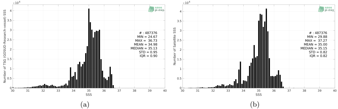
Figure 2: Histograms of SSS from TSG (GOSUD-Research-vessel) (a) and CCI SSS L4 Merged-OI v3.2 - 30-day running (ESA) (b) considering all match-up pairs per bins of 0.1 over the Tropical Pacific Ocean Pi-MEP region and for the full satellite product period.
