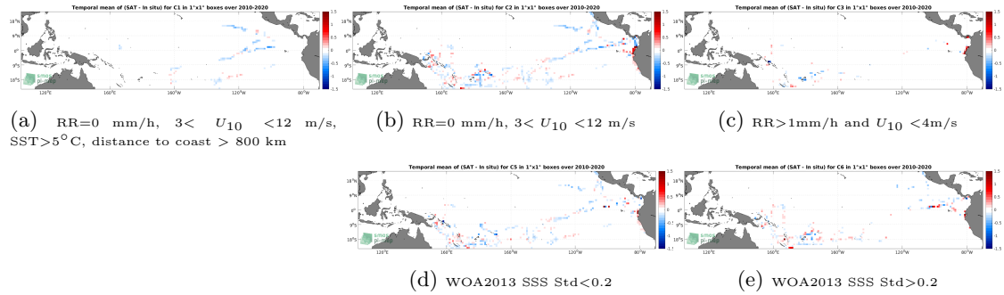
Figure 12: Temporal mean gridded over spatial boxes of size 1^{\circ}\times 1^{\circ} of \Delta SSS (CCI SSS L4 Merged-OI v3.2 - 30-day running (ESA) - TSG (GOSUD-Research-vessel)) for 5 different subdatasets corresponding to:RR=0 mm/h, 3 < U_{10} < 12 m/s, SST >5^{\circ}\text{C} , distance to coast > 800 km (a), RR=0 mm/h, 3 < U_{10} < 12 m/s (b), RR >1 mm/h and U_{10} < 4 m/s (c), WOA2013 SSS Std <0.2 (d), WOA2013 SSS Std >0.2 (e).
