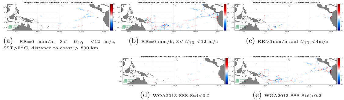
Figure 12: Temporal mean gridded over spatial boxes of size 1^\circ \times 1^\circ of \Delta SSS (CCI SSS L4 Merged-OI v3.2 - 30-day running (ESA) - TSG (GOSUD-Research-vessel)) for 5 different subdatasets corresponding to:RR=0 mm/h, 3 < U_{10} < 12 m/s, SST >5^\circ\text{C} , distance to coast > 800 km (a), RR=0 mm/h, 3 < U_{10} < 12 m/s (b), RR >1 mm/h and U_{10} < 4 m/s (c), WOA2013 SSS Std <0.2 (d), WOA2013 SSS Std >0.2 (e).
