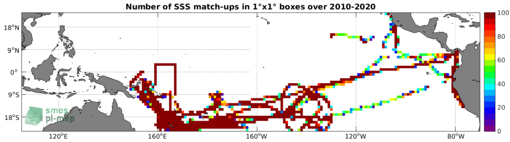
Figure 4: Number of SSS match-ups between TSG (GOSUD-Research-vessel) SSS and the CCI SSS L4 Merged-OI v3.2 - 30-day running (ESA) SSS product for the Tropical Pacific Ocean Pi-MEP region over 1^\circ \times 1^\circ boxes and for the full satellite product period.
