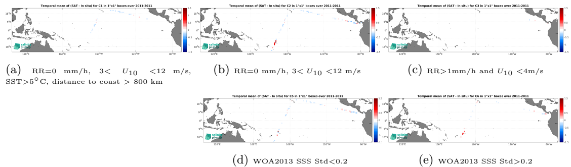
Figure 12: Temporal mean gridded over spatial boxes of size 1^\circ \times 1^\circ of \Delta SSS (CCI SSS L4 Merged-OI v3.2 - 30-day running (ESA) - TSG (CSIC-UTM)) for 5 different subdatasets corresponding to:RR=0 mm/h, 3 < U_{10} < 12 m/s, SST > 5^\circ\text{C} , distance to coast > 800 km (a), RR=0 mm/h, 3 < U_{10} < 12 m/s (b), RR > 1 mm/h and U_{10} < 4 m/s (c), WOA2013 SSS Std < 0.2 (d), WOA2013 SSS Std > 0.2 (e).
