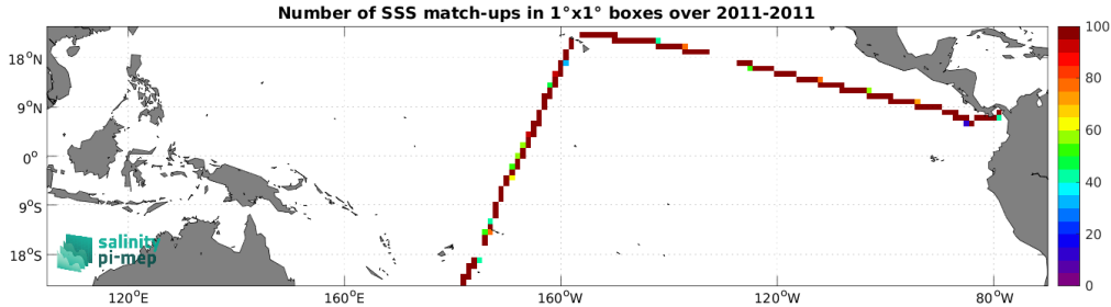
Figure 4: Number of SSS match-ups between TSG (CSIC-UTM) SSS and the CCI SSS L4 Merged-OI v3.2 - 30-day running (ESA) SSS product for the Tropical Pacific Ocean Pi-MEP region over 1^\circ \times 1^\circ boxes and for the full satellite product period.
