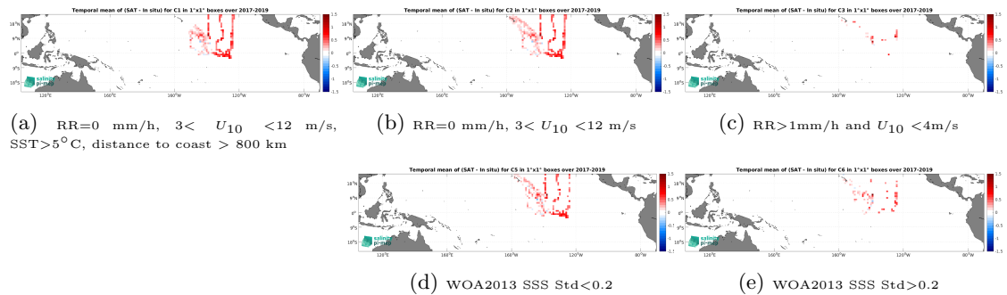
Figure 12: Temporal mean gridded over spatial boxes of size 1^\circ \times 1^\circ of \Delta SSS (CCI SSS L4 Merged-OI v3.2 - 30-day running (ESA) - Saildrone) for 5 different subdatasets corresponding to: RR=0 mm/h, 3 < U_{10} < 12 m/s, SST > 5^\circ\text{C} , distance to coast > 800 km (a), RR=0 mm/h, 3 < U_{10} < 12 m/s (b), RR > 1 mm/h and U_{10} < 4 m/s (c), WOA2013 SSS Std < 0.2 (d), WOA2013 SSS Std > 0.2 (e).
