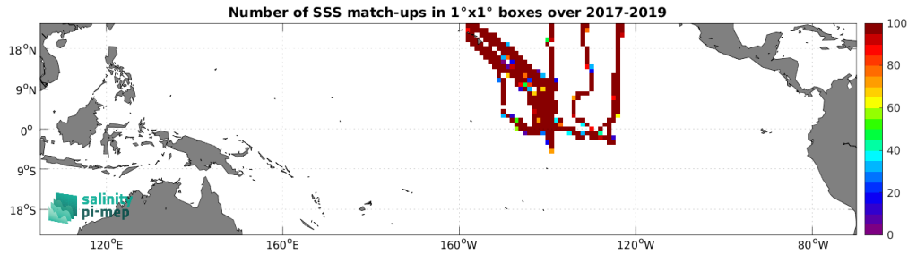
Figure 4: Number of SSS match-ups between Sailldrone SSS and the CCI SSS L4 Merged-OI v3.2 - 30-day running (ESA) SSS product for the Tropical Pacific Ocean Pi-MEP region over 1^\circ \times 1^\circ boxes and for the full satellite product period.
