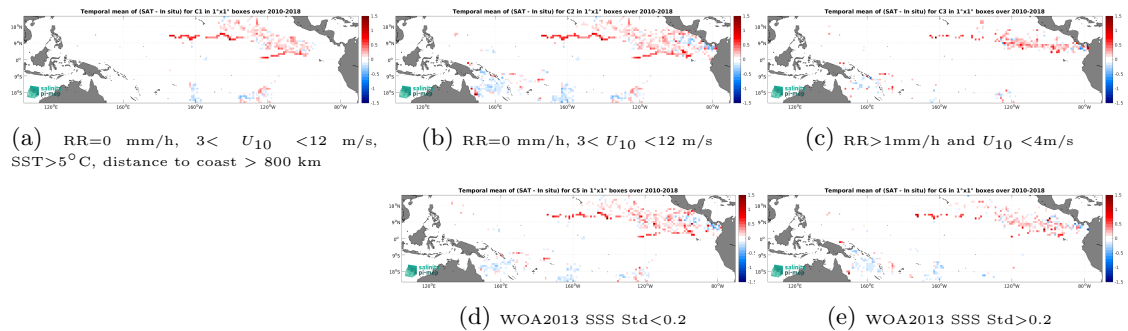
Figure 11: Temporal mean gridded over spatial boxes of size 1^\circ \times 1^\circ of \Delta SSS (CCI SSS L4 Merged-OI v3.2 - 30-day running (ESA) - Surface drifters) for 5 different subdatasets corresponding to:RR=0 mm/h, 3 < U_{10} < 12 m/s, SST > 5^\circ\text{C} , distance to coast > 800 km (a), RR=0 mm/h, 3 < U_{10} < 12 m/s (b), RR > 1 mm/h and U_{10} < 4 m/s (c), WOA2013 SSS Std < 0.2 (d), WOA2013 SSS Std > 0.2 (e).
