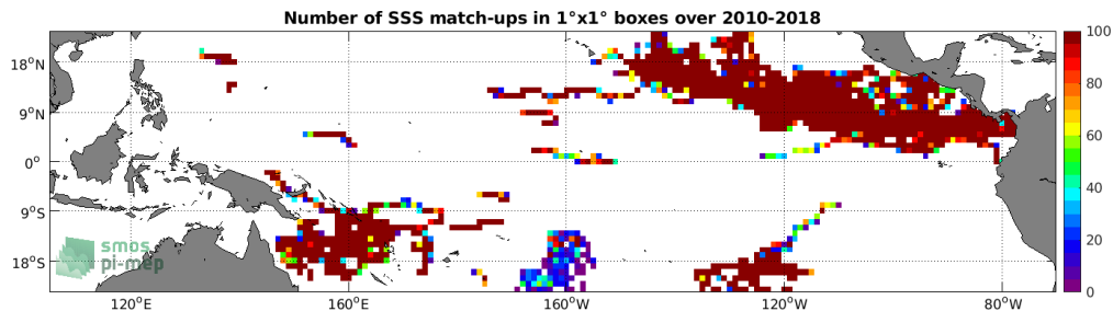
Figure 3: Number of SSS match-ups between Surface drifters SSS and the CCI SSS L4 Merged-OI v3.2 - 30-day running (ESA) SSS product for the Tropical Pacific Ocean Pi-MEP region over 1^\circ \times 1^\circ boxes and for the full satellite product period.
