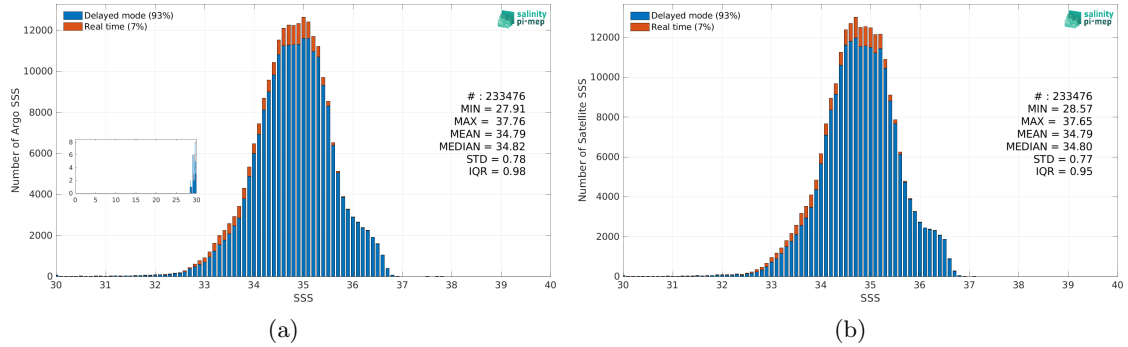
Figure 2: Histograms of SSS from Argo (a) and CCI SSS L4 Merged-OI v3.2 - 30-day running (ESA) (b) considering all match-up pairs per bins of 0.1 over the Tropical Pacific Ocean Pi-MEP region and for the full satellite product period.
