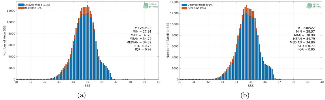
Figure 2: Histograms of SSS from Argo (a) and CCI SSS L4 Merged-OI v3.2 - 30-day running (ESA) (b) considering all match-up pairs per bins of 0.1 over the Tropical Pacific Ocean Pi-MEP region and for the full satellite product period.
