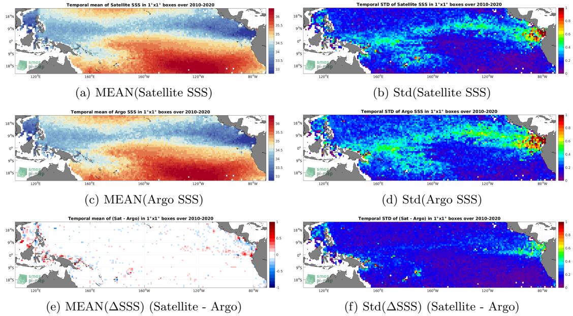
Figure 6: Temporal mean (left) and Std (right) of SSS from CCI SSS L4 Merged-OI v3.2 - 30-day running (ESA) (top), Argo (middle), and of \Delta SSS (Satellite - Argo). Only match-up pairs are used to generate these maps.
