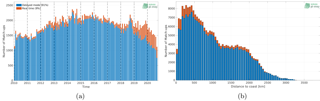
Figure 1: Number of match-ups between Argo and CCI SSS L4 Merged-OI v3.2 - 30-day running (ESA) SSS as a function of time (a) and as function of the distance to coast (b) over the Tropical Pacific Ocean Pi-MEP region and for the full satellite product period.
