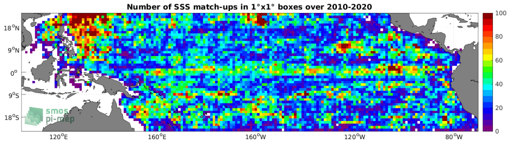
Figure 4: Number of SSS match-ups between Argo SSS and the CCI SSS L4 Merged-OI v3.2 - 30-day running (ESA) SSS product for the Tropical Pacific Ocean Pi-MEP region over 1^\circ \times 1^\circ boxes and for the full satellite product period.
