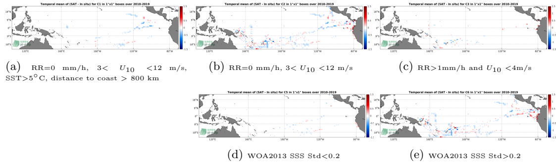
Figure 12: Temporal mean gridded over spatial boxes of size 1^\circ \times 1^\circ of \Delta SSS (CCI SSS L4 Merged-OI v2.31 - 7-day running (ESA) - TSG (GOSUD-Research-vessel)) for 5 different subdatasets corresponding to:RR=0 mm/h, 3 < U_{10} < 12 m/s, SST >5^\circ\text{C} , distance to coast > 800 km (a), RR=0 mm/h, 3 < U_{10} < 12 m/s (b), RR >1 mm/h and U_{10} < 4 m/s (c), WOA2013 SSS Std <0.2 (d), WOA2013 SSS Std >0.2 (e).
