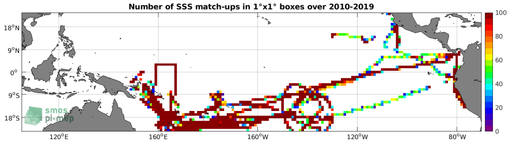
Figure 4: Number of SSS match-ups between TSG (GOSUD-Research-vessel) SSS and the CCI SSS L4 Merged-OI v2.31 - 7-day running (ESA) SSS product for the Tropical Pacific Ocean Pi-MEP region over 1^\circ \times 1^\circ boxes and for the full satellite product period.
