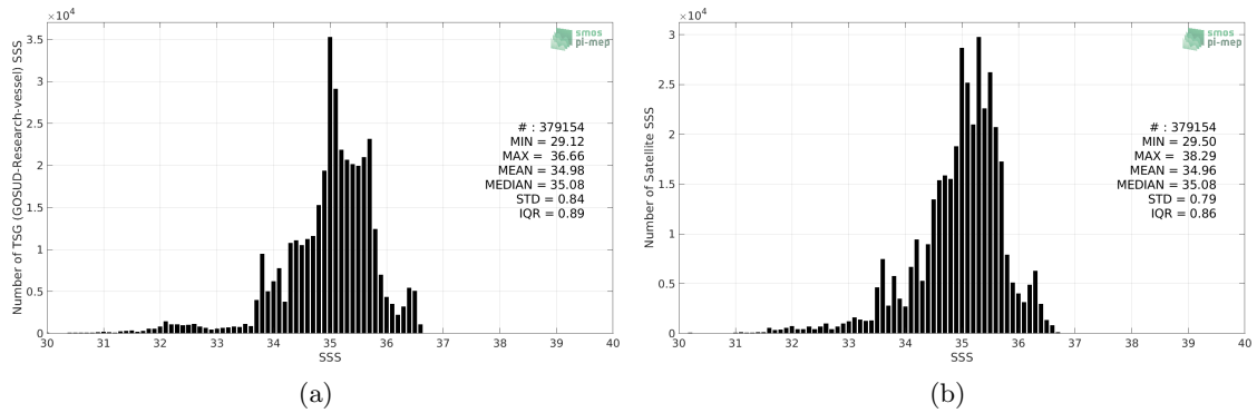
Figure 2: Histograms of SSS from TSG (GOSUD-Research-vessel) (a) and CCI SSS L4 Merged-OI v2.31 - 7-day running (ESA) (b) considering all match-up pairs per bins of 0.1 over the Tropical Pacific Ocean Pi-MEP region and for the full satellite product period.
