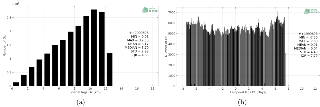
Figure 5: Histograms of the spatial (a) and temporal (b) lags between the location/time of the TSG (SAMOS) measurement and the date of the corresponding CCI SSS L4 Merged-OI v2.31 - 30-day running (ESA) SSS pixel.
